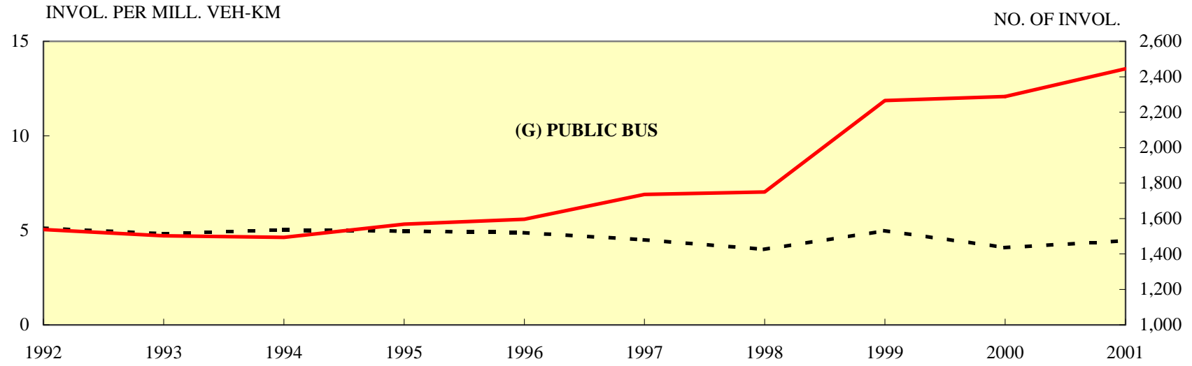
FIGURE 1.13 (CONT'D) - MOTOR VEHICLE INVOLVEMENT RATE BY CLASS (1992 - 2001)
