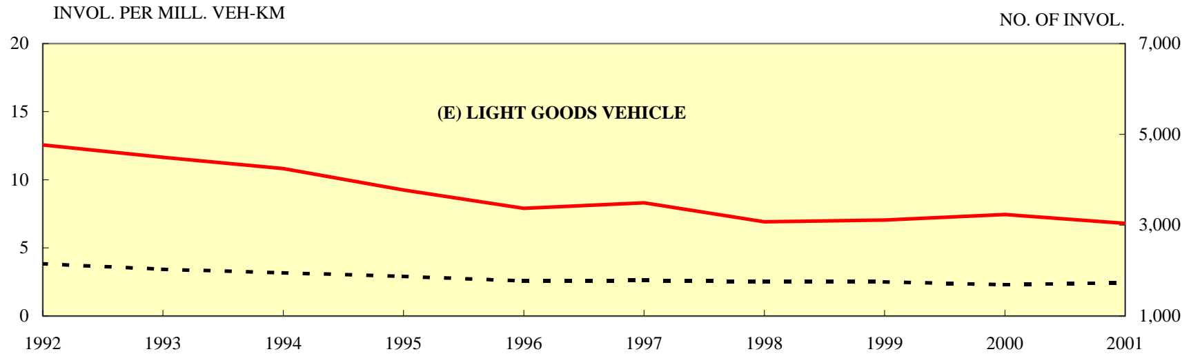
FIGURE 1.13 (CONT'D) - MOTOR VEHICLE INVOLVEMENT RATE BY CLASS (1992 - 2001)
