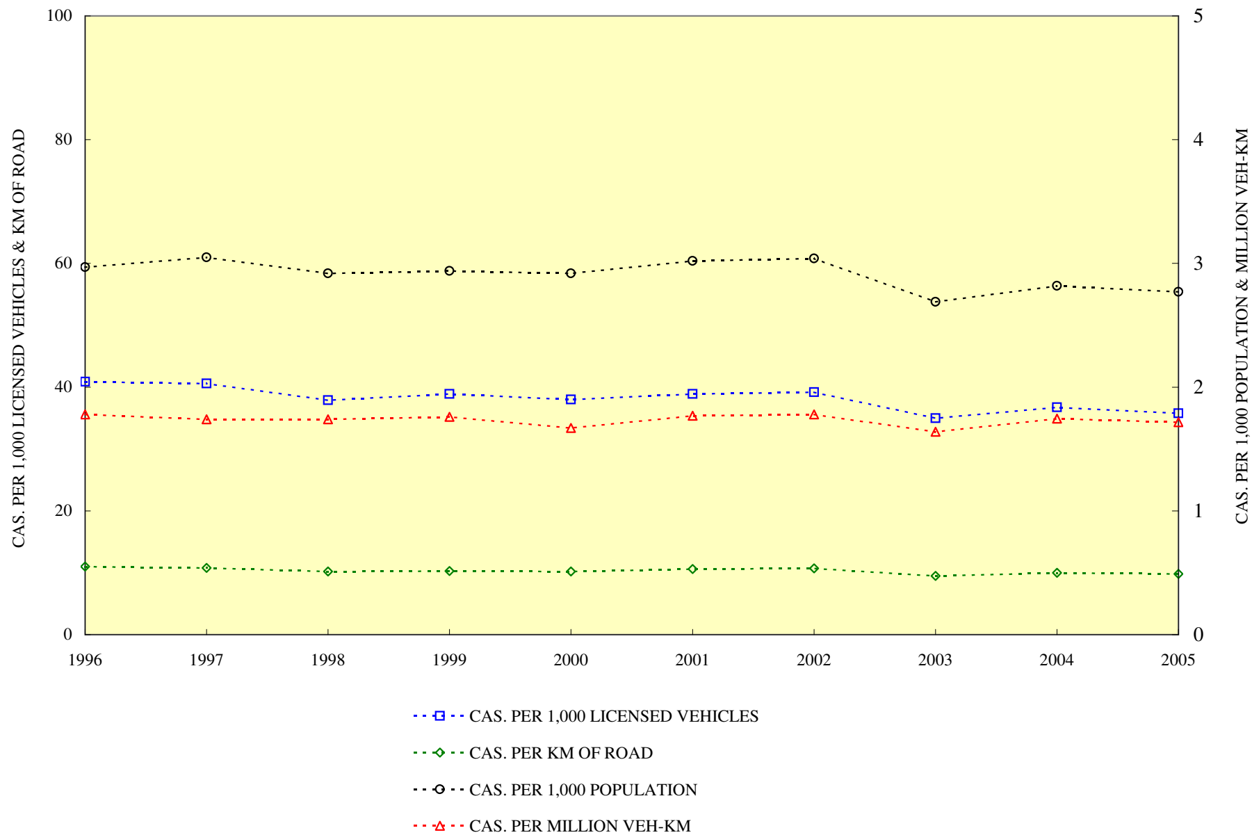
FIGURE 1.23 - CHANGES IN ROAD TRAFFIC CASUALTY RATES (1996 - 2005)
