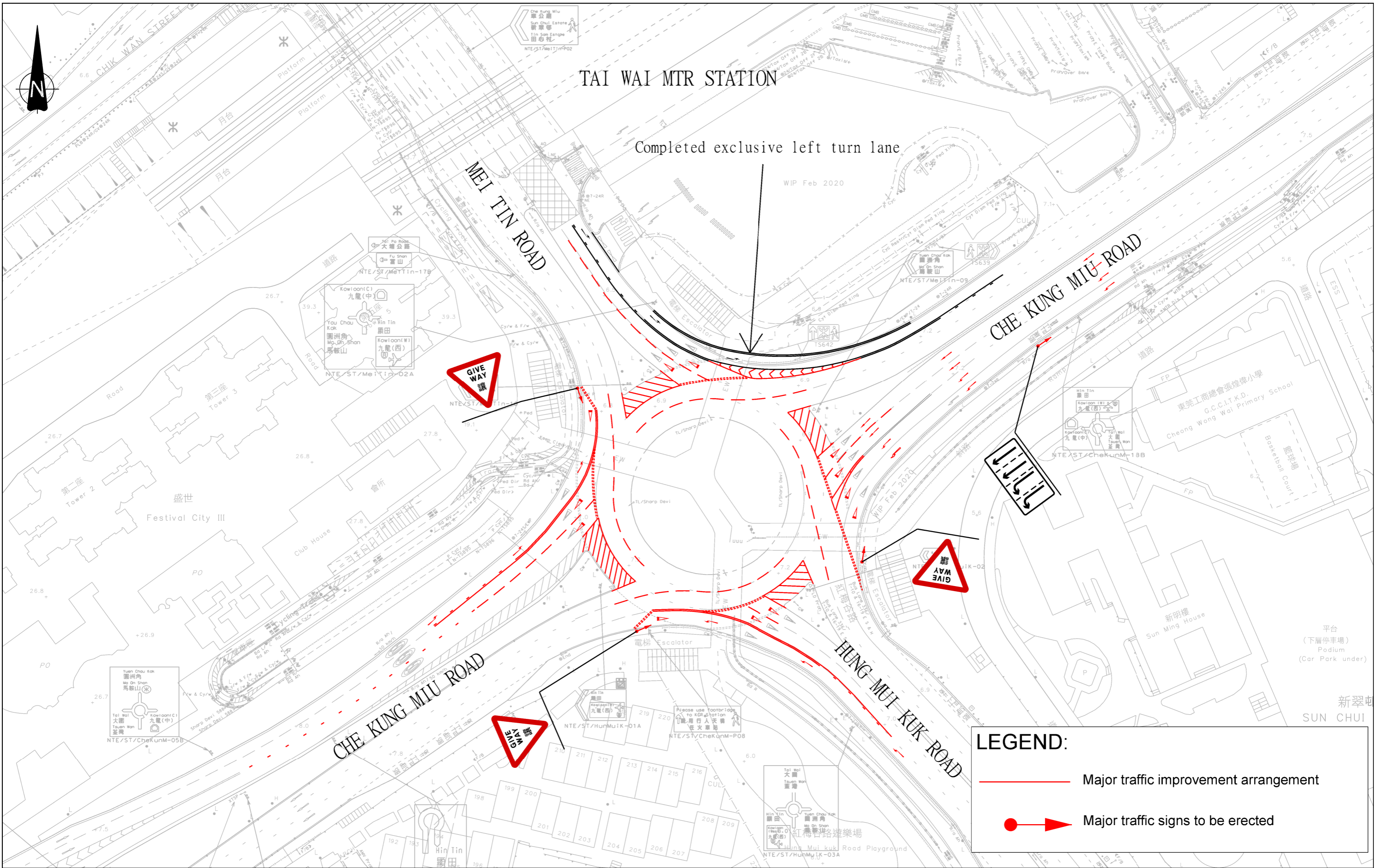
MEI TIN ROAD/CHE KUNG MIU ROAD/HUNG MUI KUK ROAD ROUNDABOUT IMPROVEMENT SCHEME DRAWING
