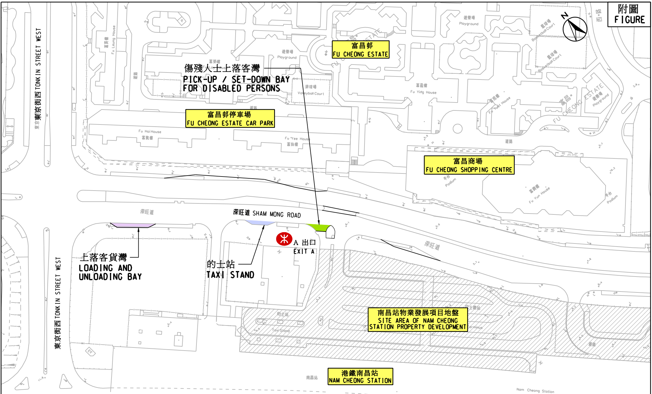
深水埗深旺道遷移的士站及上落客貨設施 RELOCATION OF TAXI STAND AND LOADING / UNLOADING FACILITIES ON SHAM MONG ROAD, SHAM SHUI PO
