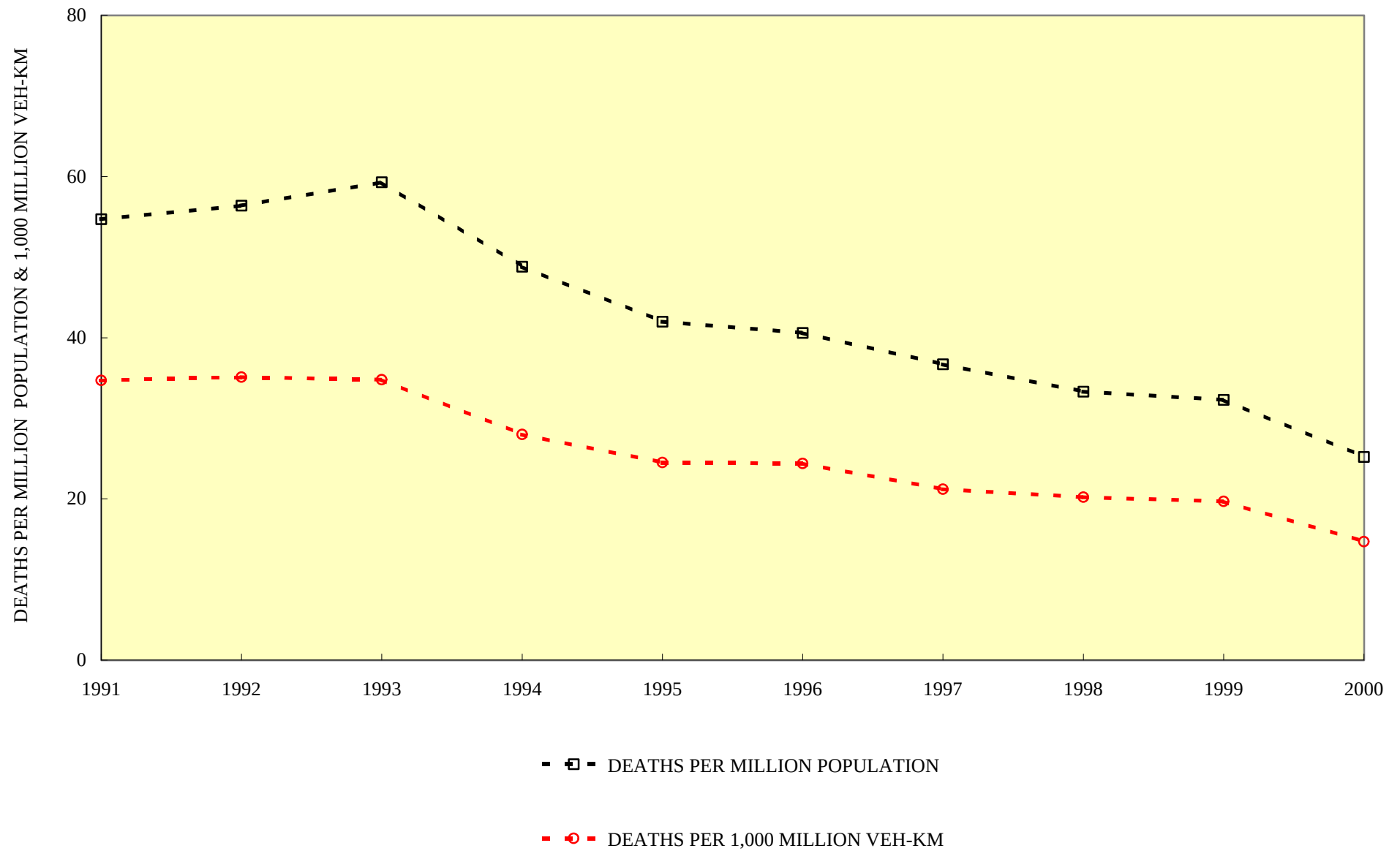
FIGURE 1.30 - CHANGES IN ROAD TRAFFIC FATALITY RATES (1991 - 2000)
