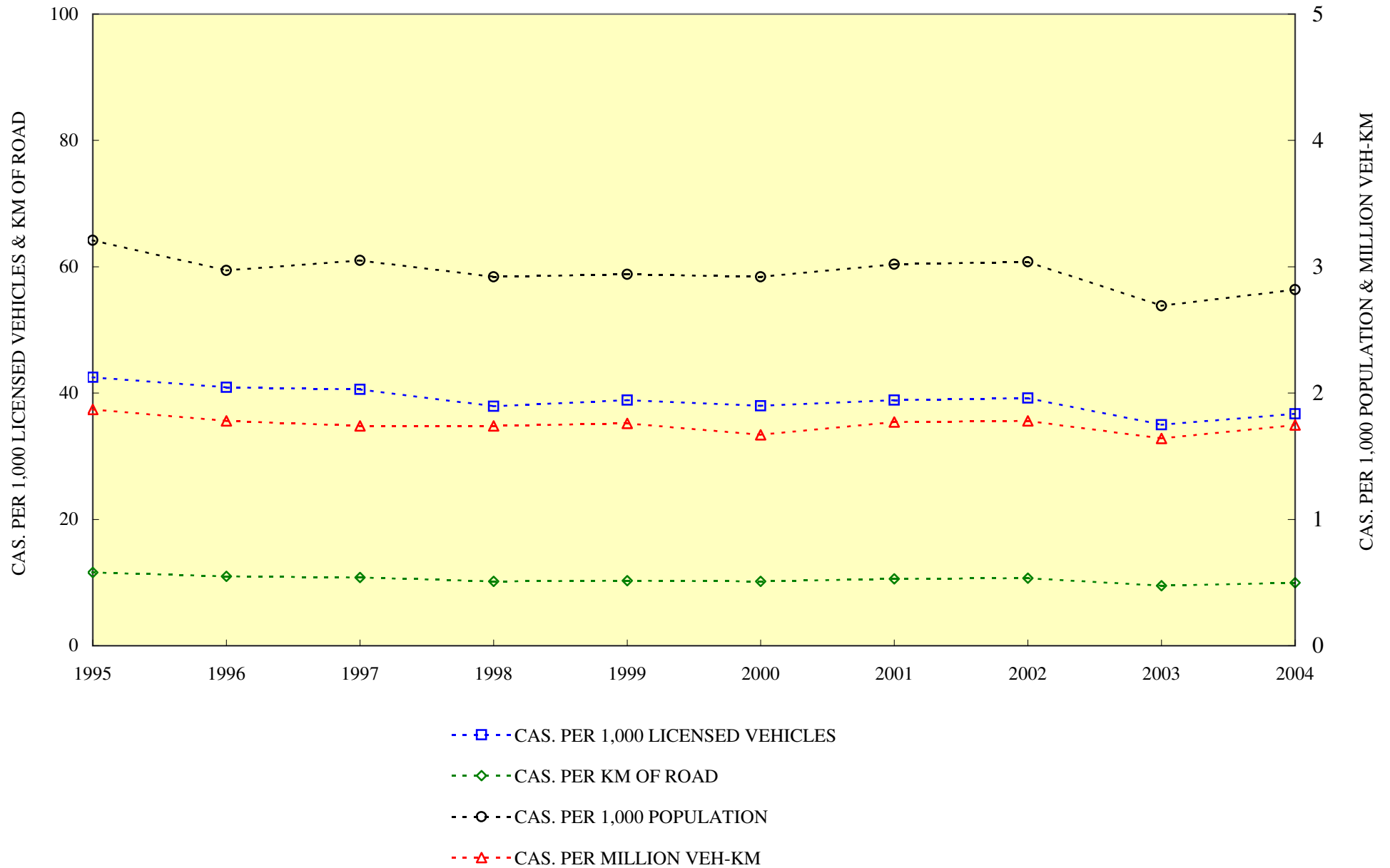
FIGURE 1.23 - CHANGES IN ROAD TRAFFIC CASUALTY RATES (1995 - 2004)
