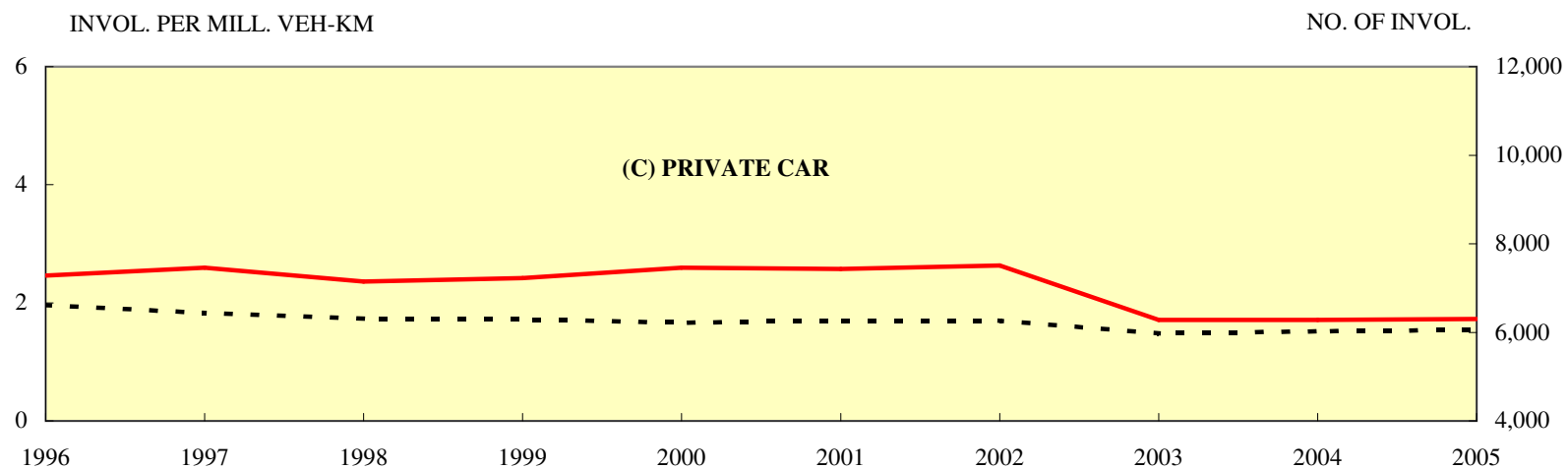
FIGURE 1.13 (CONT'D) - MOTOR VEHICLE INVOLVEMENT RATE BY CLASS (1996 - 2005)
