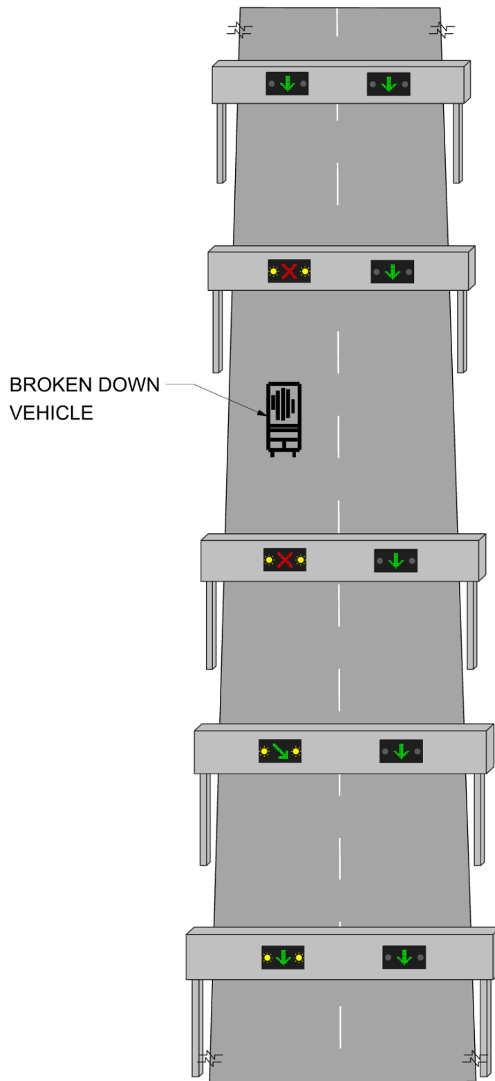
DIAGRAM 5.4.3: LANE CLOSURE
