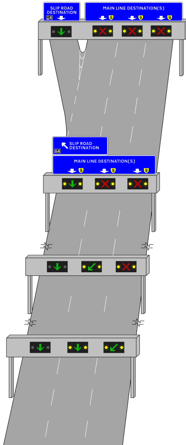
DIAGRAM 5.4.4: CARRIAGEWAY CLOSURE
