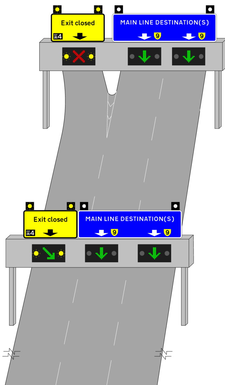
DIAGRAM 5.6.1 : EXIT CLOSURE
