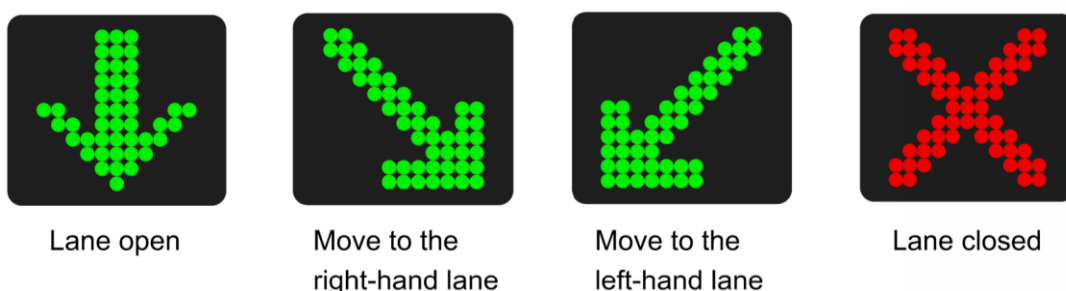
DIAGRAM 5.4.2: LANE SIGNAL ASPECTS
