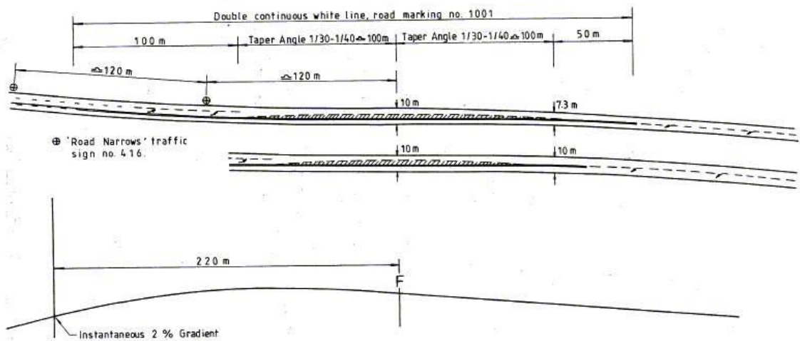
DIAGRAM 3.3.8.3 : END OF CLIMBING LANE
