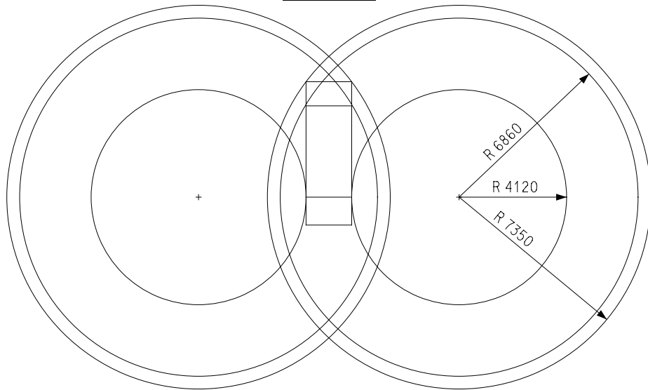
DIAGRAM 2.2.3.2 : TURNING CIRCLE PRIVATE CAR (LARGE SIZE) 5.49 x 1.88
