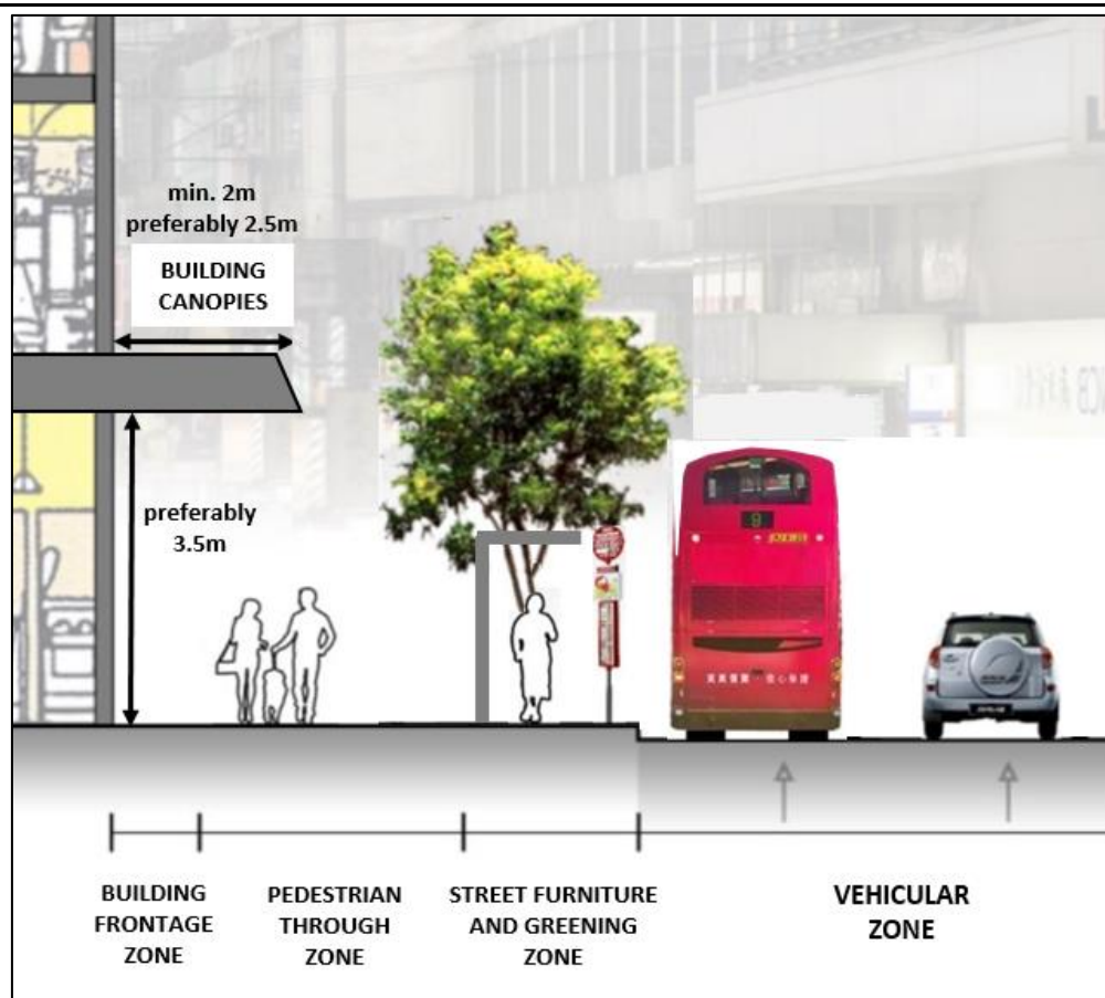
DIAGRAM 3.4.11.1 : PROTOTYPE OF THE THREE-ZONE CONCEPT OF FOOTWAYS
