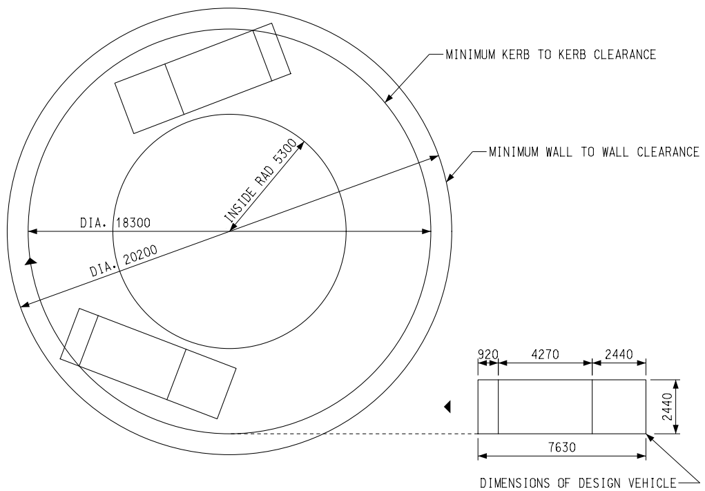
DIAGRAM 2.2.3.3 : RECOMMENDED MINIMUM STANDARDS OF TURNING CIRCLE AND TURNTABLE FOR GOODS VEHICLES MIN. STANDARD TURNING CIRCLE FOR GOODS VEHICLE
