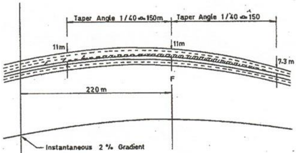
DIAGRAM 3.3.9.4 : END OF DUAL CARRIAGEWAY CLIMBING LANE
