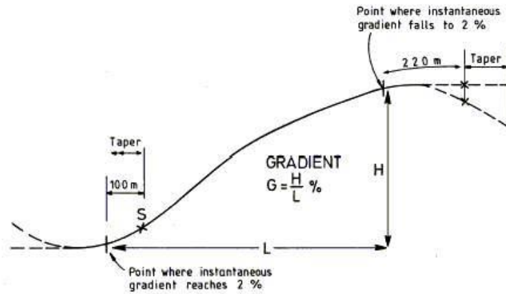
DIAGRAM 3.3.8.2 : START OF CLIMBING LANE
