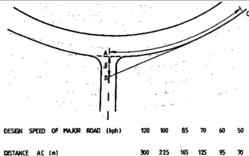
DIAGRAM 4.3.8.1 : VISIBILITY SPLAYS AT PRIORITY JUNCTIONS
