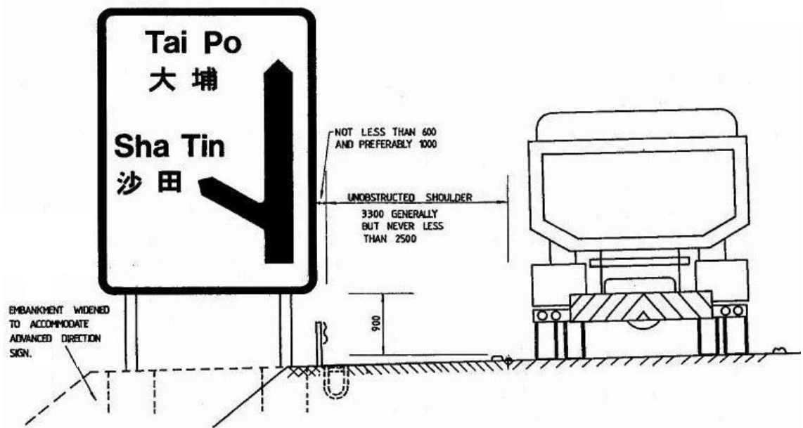
DIAGRAM 6.4.1.5: LOCATION OF LARGE ROAD SIGN
