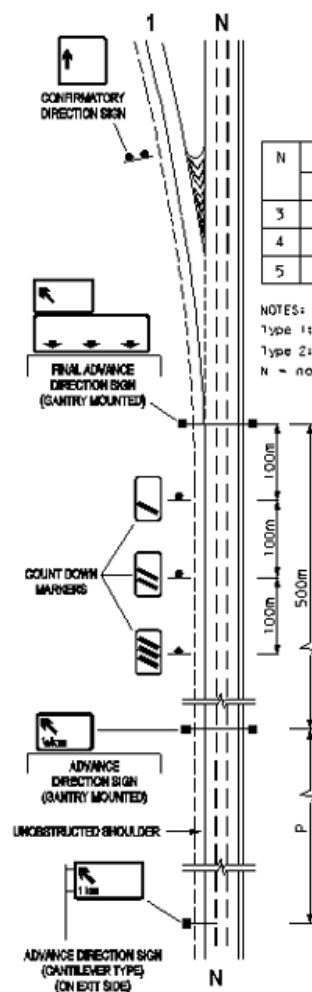
(a) Layout for Gantry Signs
