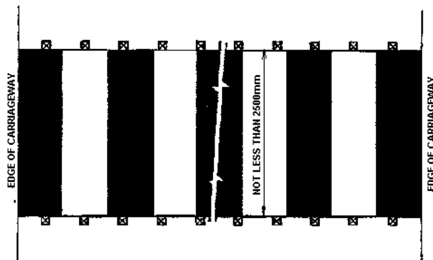
DIAGRAM 3.7.3.1 : INDICATION OF ZEBRA PEDESTRIAN CROSSING
