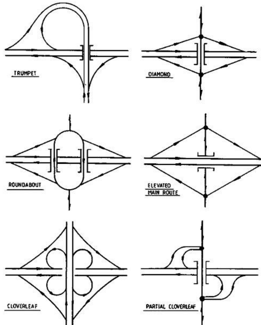
DIAGRAM 4.6.2.1 : TYPES OF GRADE SEPARATED INTERCHANGE
