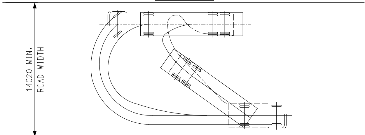
DIAGRAM 2.2.3.6 : 90° & 180° TURNING CONTAINER 180° TURNING
