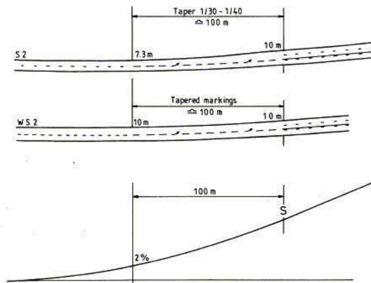
DIAGRAM 3.3.8.2 : START OF CLIMBING LANE
