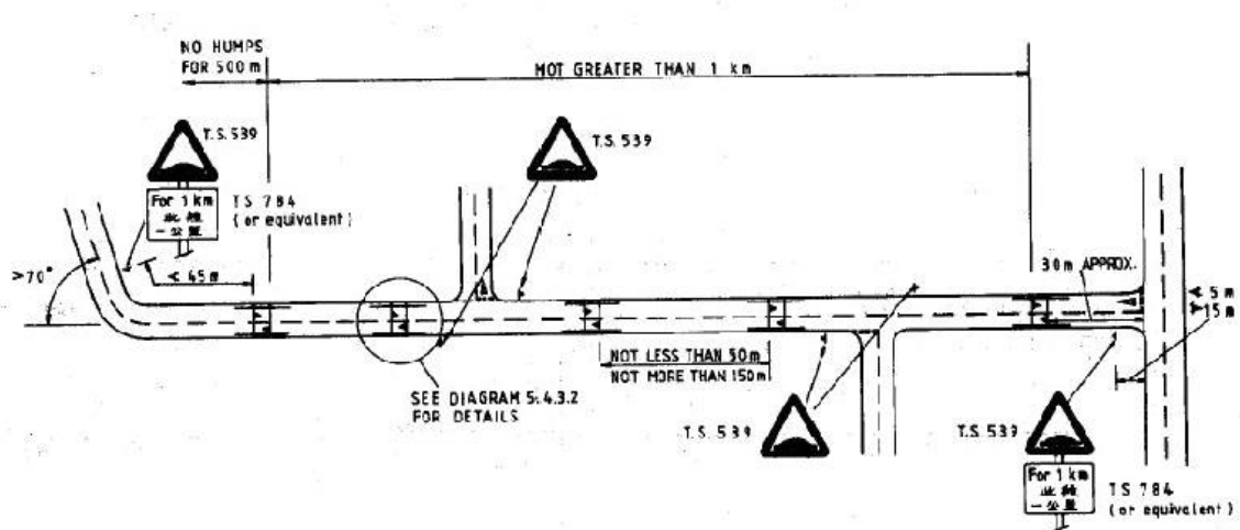
DIAGRAM 5.4.3.3 : ROAD HUMP INSTALLATION
