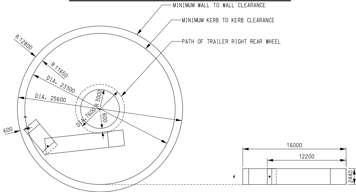
DIAGRAM 2.2.3.5 : CONTAINER TURNING CIRCLES
