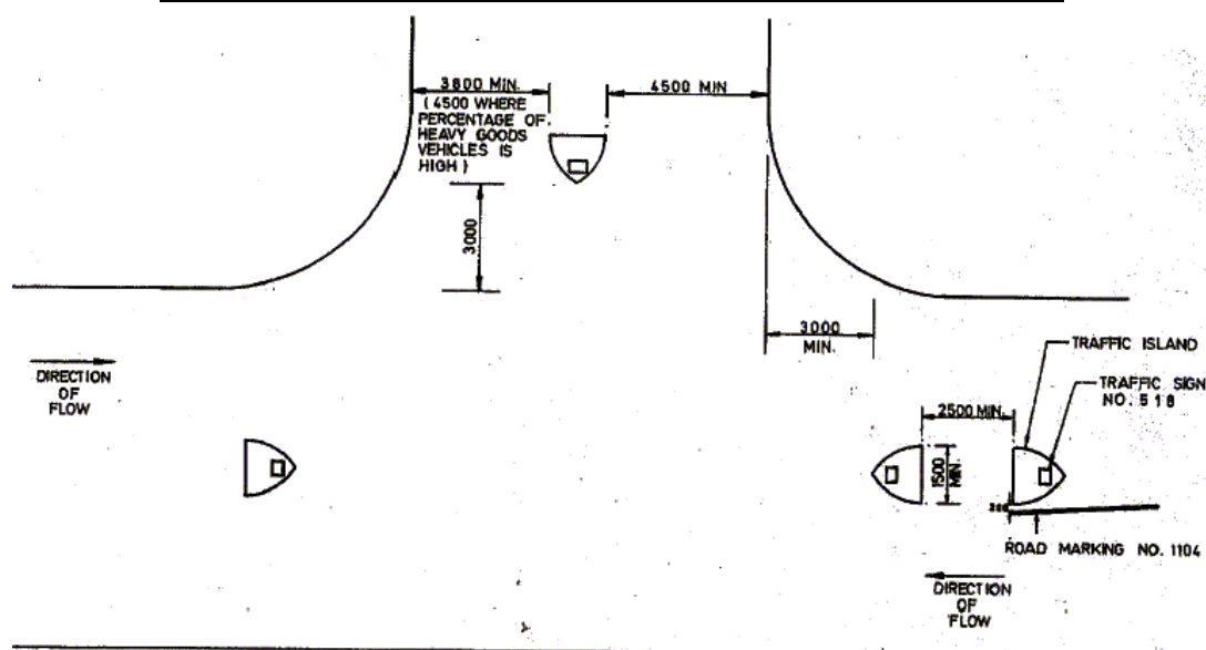
DIAGRAM 3.4.7.1 : TRAFFIC ISLANDS AT TEE JUNCTIONS
