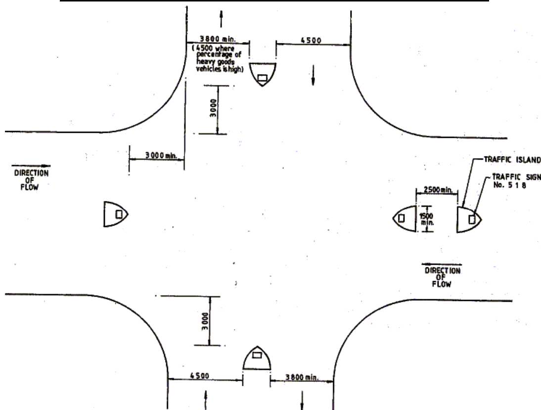
DIAGRAM 3.4.7.2 : TRAFFIC ISLANDS AT 4 - WAY JUNCTIONS
