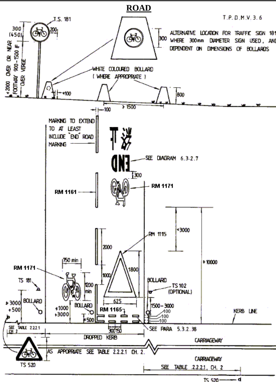
DIAGRAM 6.3.2.1 : START AND END OF CYCLE TRACK AT A JUNCTION WITH A
