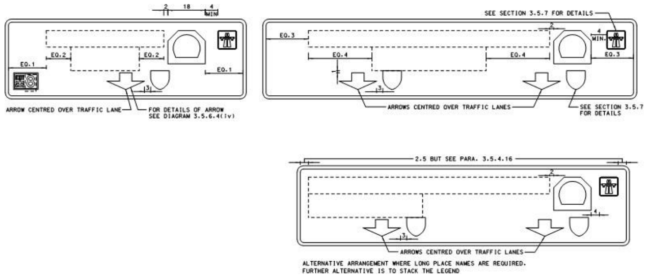
DIAGRAM 3.5.6.13 : LOCATION OF TUNNEL SYMBOL ON GANTRY SIGNS DIMENSIONS IN STROKE WIDTHS
