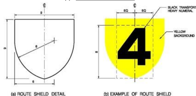
DIAGRAM 3.5.7.1: ROUTE SHIELDS DIMENSIONS IN STROKE WIDTHS
