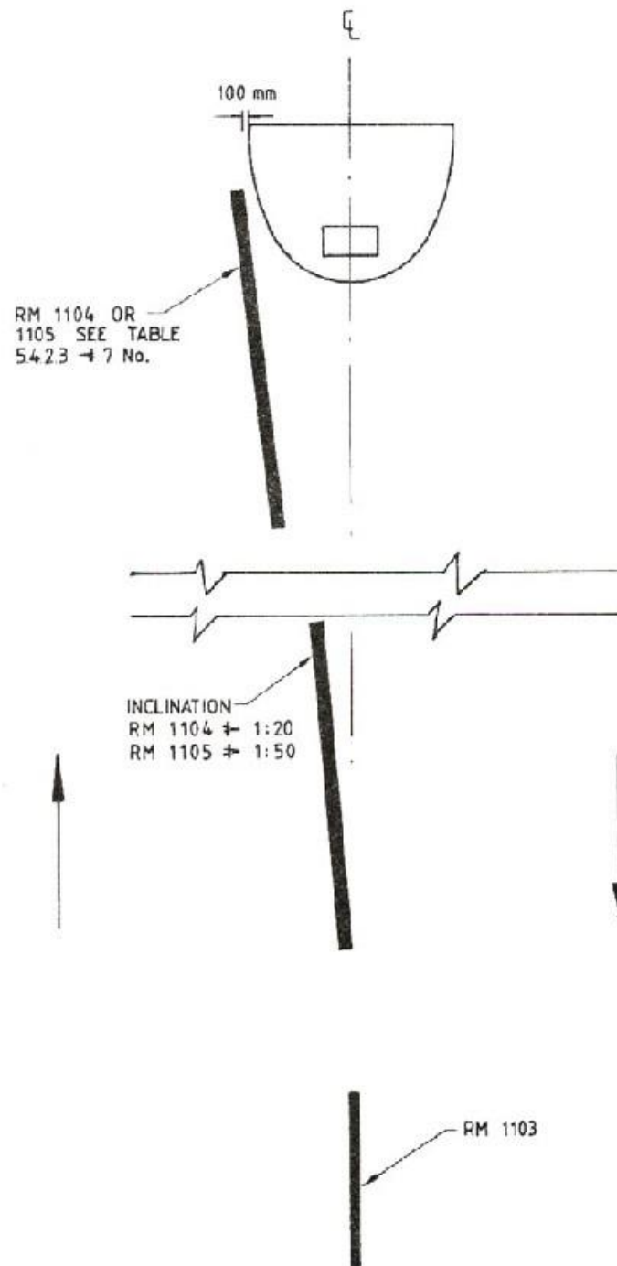
DIAGRAM 5.4.2.1 : INCLINED WARNING LINE AT REFUGES
