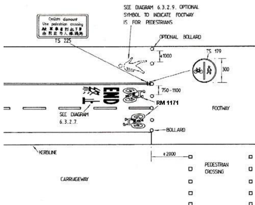
DIAGRAM 6.3.2.11 : START / TERMINATION OF A CYCLE TRACK NEAR A PEDESTRIAN CROSSING
