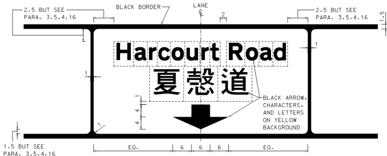
DIAGRAM 3.6.9.1 : GANTRY DIRECTIONAL SIGN DIMENSIONS IN STROKE WIDTHS
