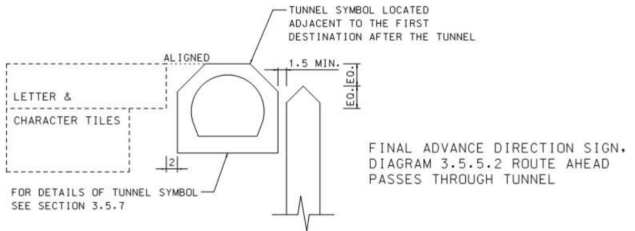
DIAGRAM 3.5.5.3 : LOCATION OF TUNNEL SYMBOL FOR DIAGRAMS 3.5.5.1 & 3.5.5.2 DIMENSIONS IN STROKE WIDTHS
