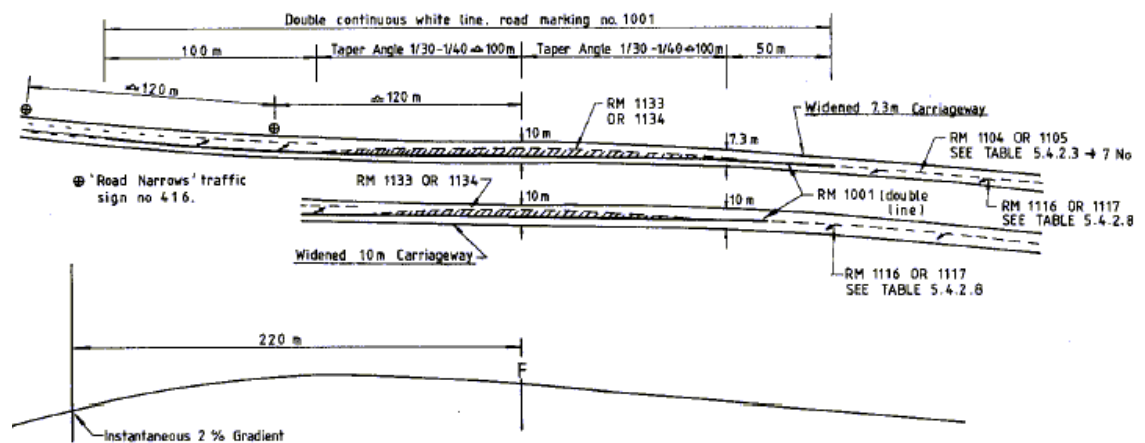
DIAGRAM 5.3.2.6 : MARKINGS FOR END OF CARRIAGEWAY ( SEE ALSO SECTION 3.3.8 CHAPTER 3 VOLUME 2 )
