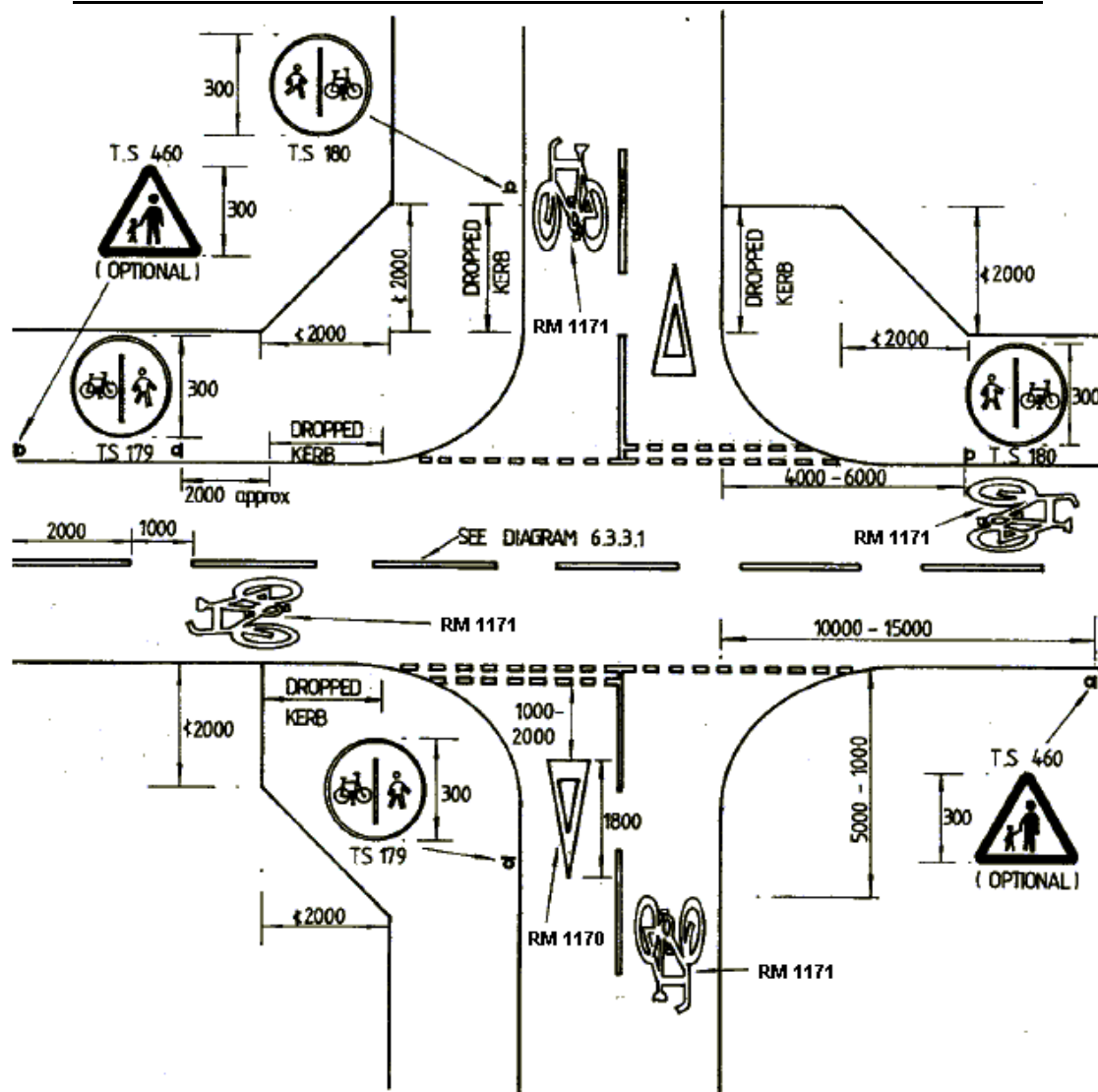
DIAGRAM 6.3.3.4 : CYCLE TRACK / FOOTWAY FOUR-WAY JUNCTION
