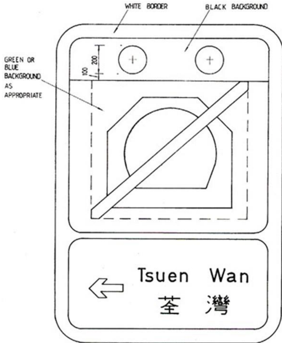
DIAGRAM 4.5.5.9 : FREE STANDING "TUNNEL CLOSED" SIGN INCOPRORATING DIVERSIONARY SIGNING
