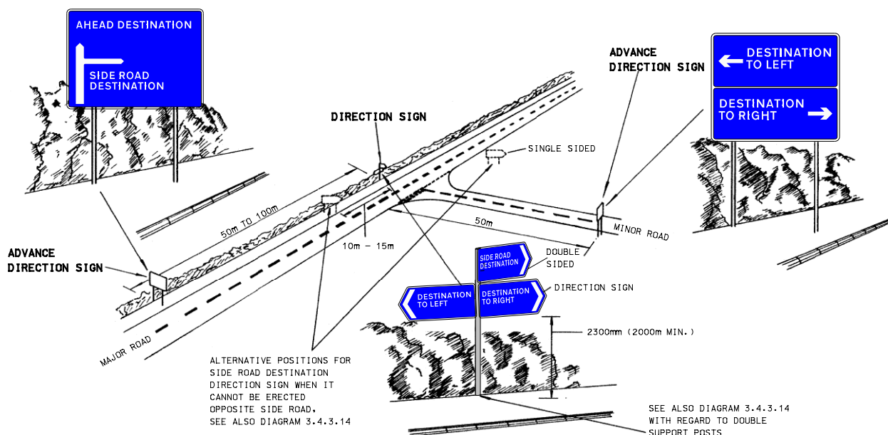
DIAGRAM 3.4.3.2 : USE OF ADVANCE DIRECTION AND DIRECTION SIGNS AT “T” JUNCTION
