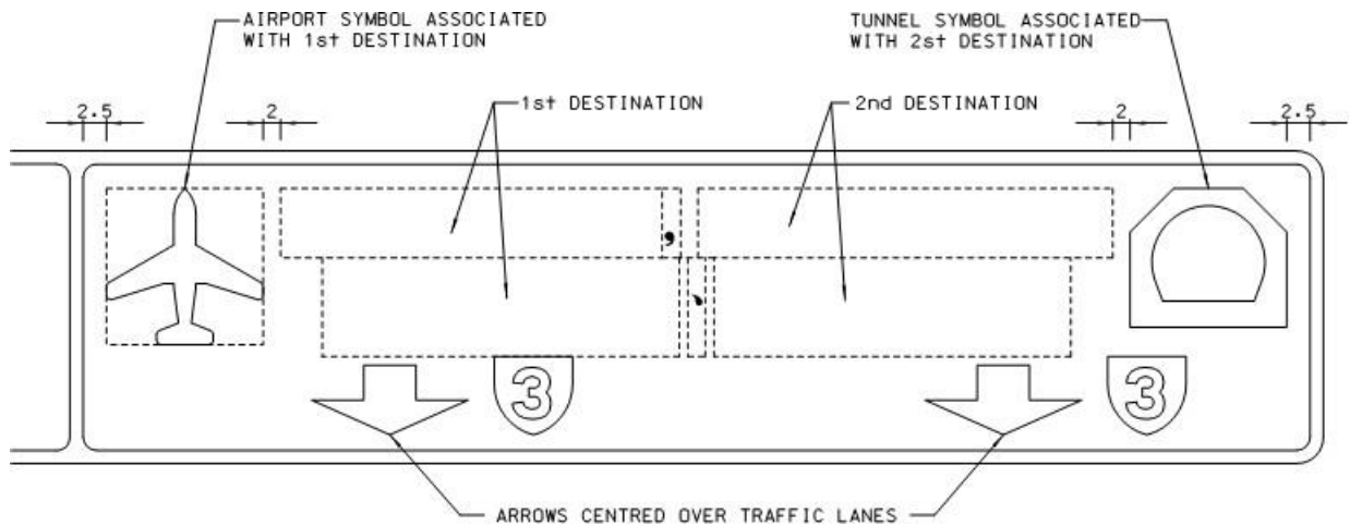
DIAGRAM 3.5.7.10 : ARRANGEMENT OF SYMBOLS ADJACENT TO ASSOCIATED DESTINATIONS ON THE SAME LINE DIMENSIONS IN STROKE WIDTHS
