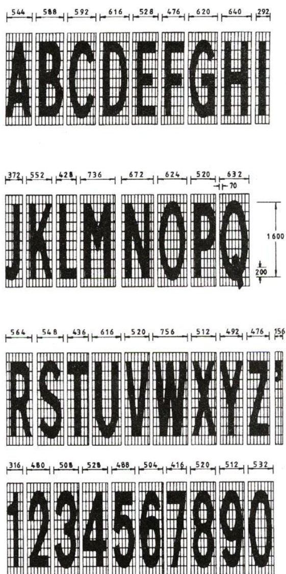
DIAGRAM 5.8.4.1 : “1600 mm” HEIGHT LETTERS AND NUMERALS
