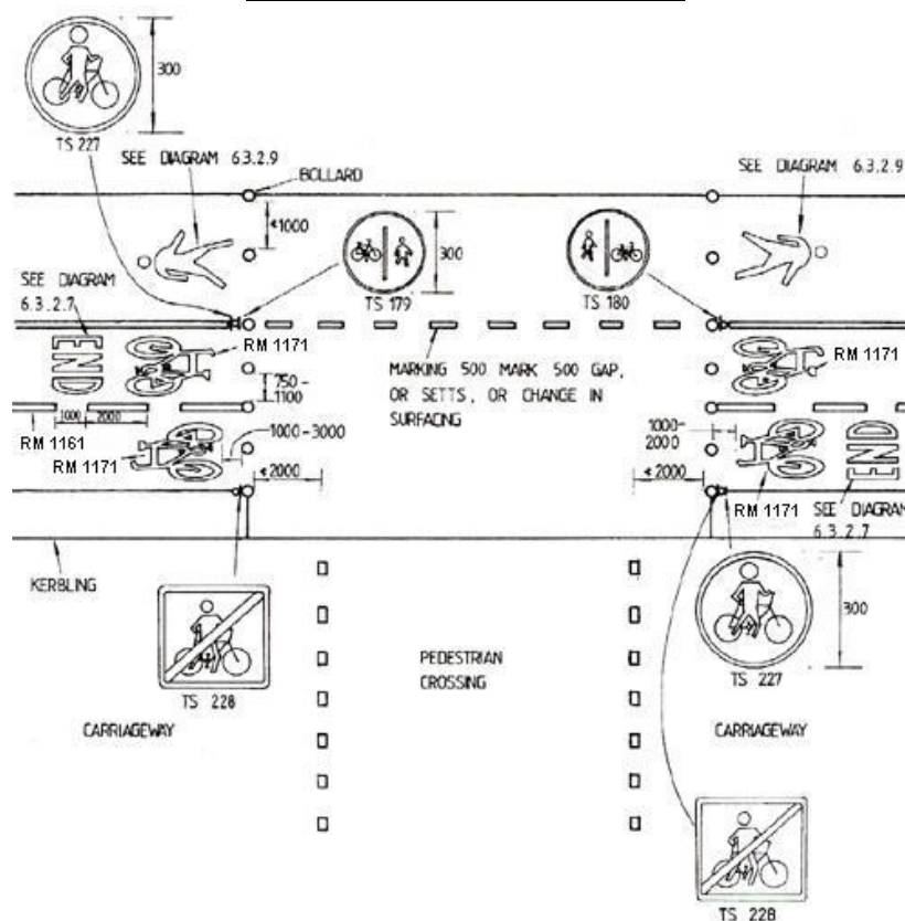
DIAGRAM 6.3.2.10 : DUAL START / TERMINATION OF CYCLE TRAC IN THE VICINITY OF PEDESTRIAN CROSSING
