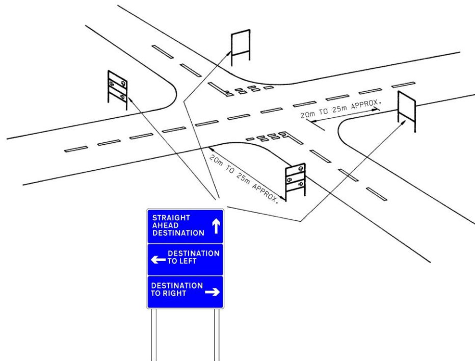
DIAGRAM 3.4.3.15 : DIRECTIONAL SIGNING FOR A FOUR-WAY, LOW VOLUME, LOW APPROACH SPEED JUNCTION
