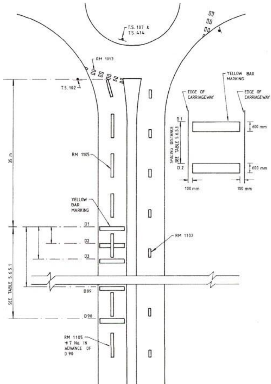
DIAGRAM 5.6.5.5 : YELLOW TRANSVERSE BAR MARKINGS AT APPROACH TO ROUNDABOUTS
