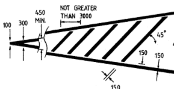
RM 1037 (TC 513)
