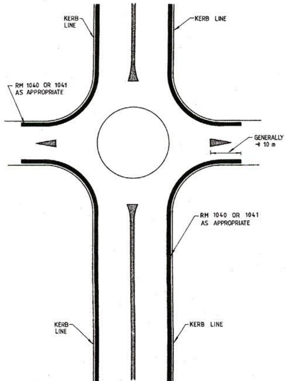
DIAGRAM 5.3.2.13 : STOPPING RESTRICTION MARKINGS AT ROUNDABOUTS
