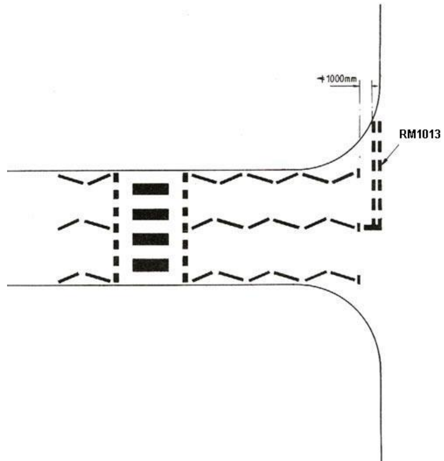
DIAGRAM 5.7.2.4 : ZEBRA CROSSING NEAR JUNCTION WITH MAJOR ROAD
