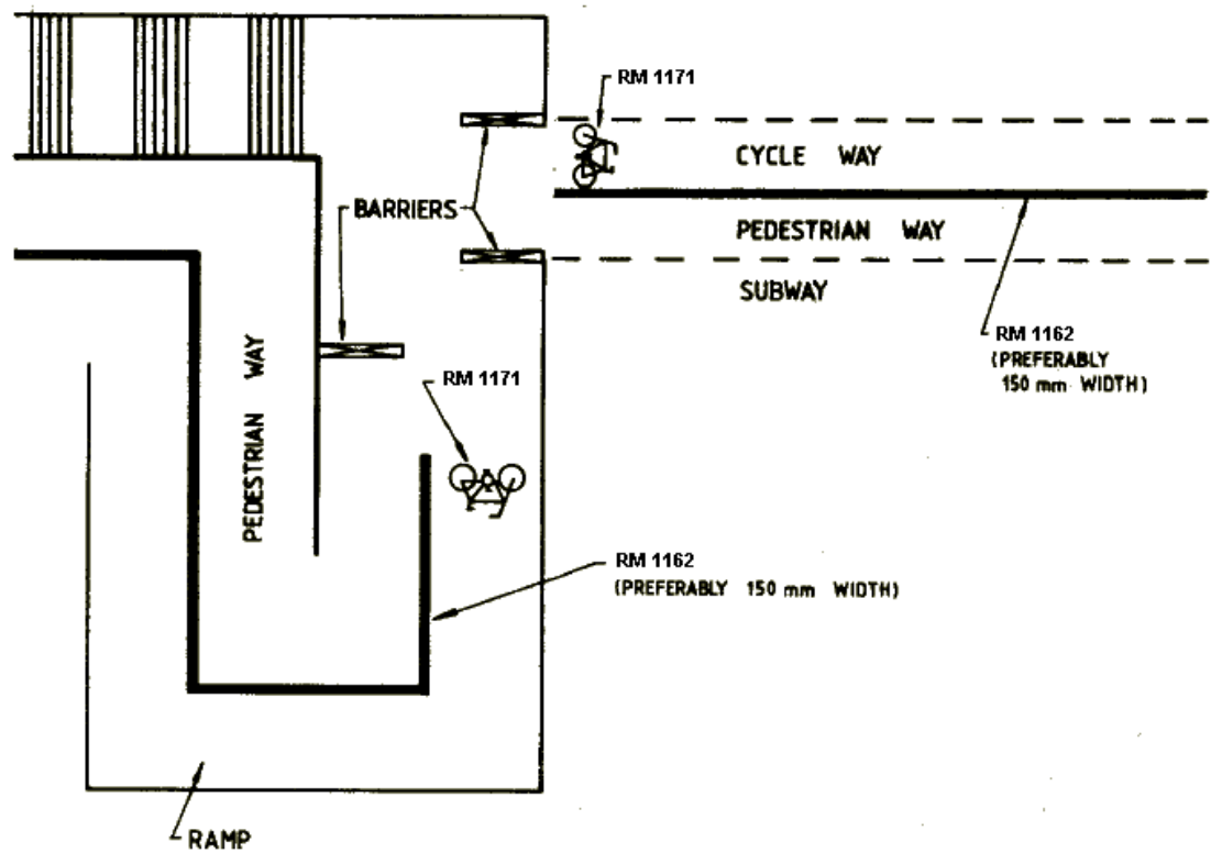
DIAGRAM 5.7.5.1 : CYCLE WAY MARKINGS FOR SUBWAYS AND FOOTBRIDGES
