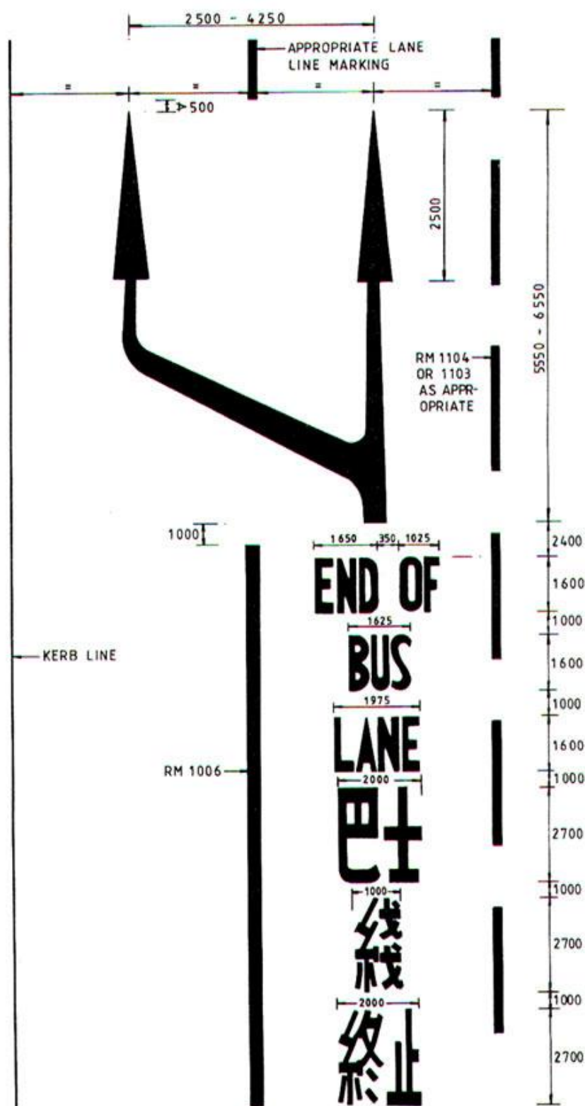
DIAGRAM 5.8.2.4 : END OF BUS LANE MARKINGS
