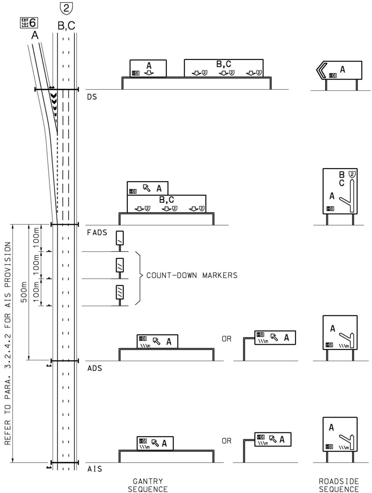
DIAGRAM 3.4.2.1 : SIGNING ARRANGEMENT FOR TAPER DIVERGE JUNCTION
