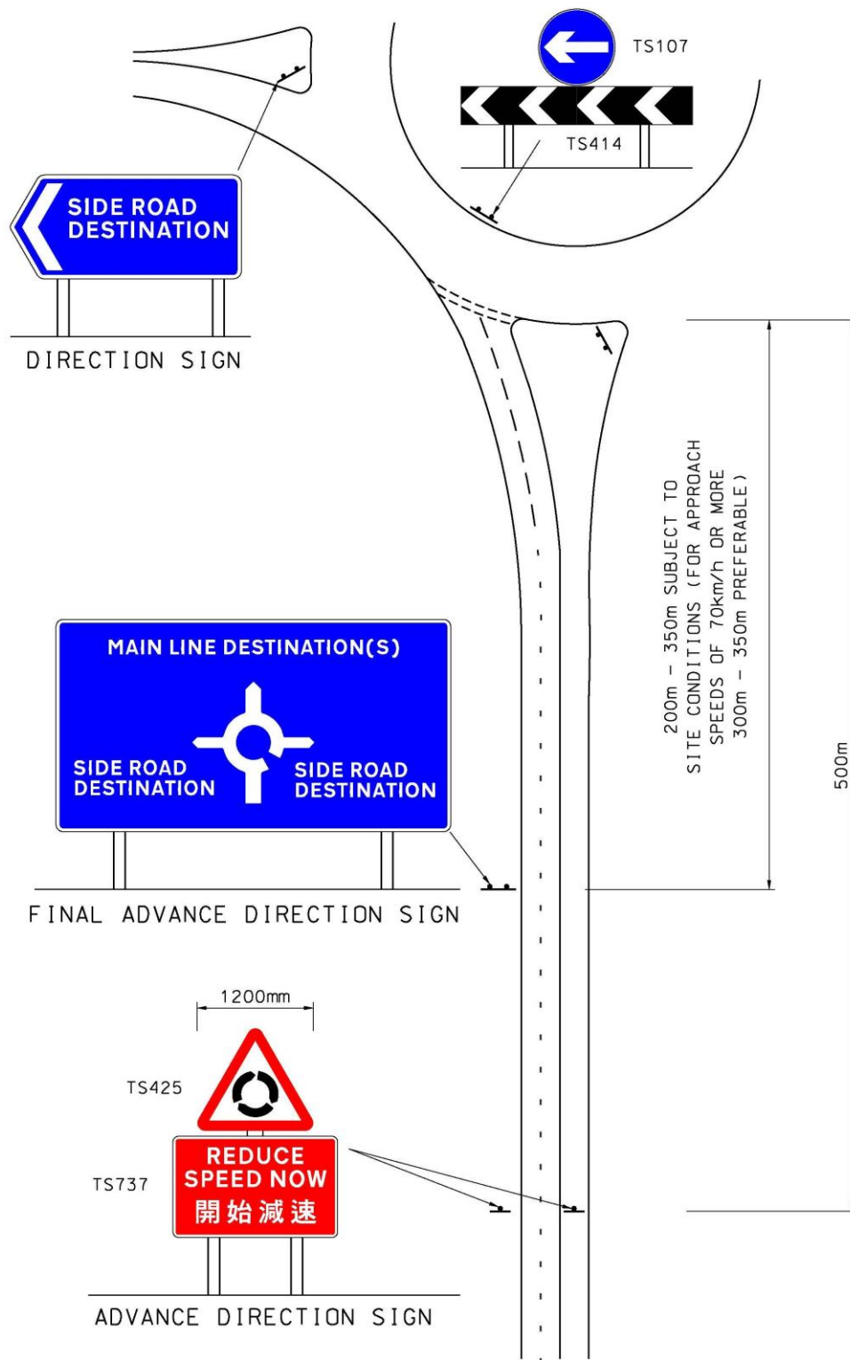
DIAGRAM 3.4.2.20 : DIRECTIONAL SIGNING FOR ROUNDABOUTS WITH HIGH SPEED APPROACH
