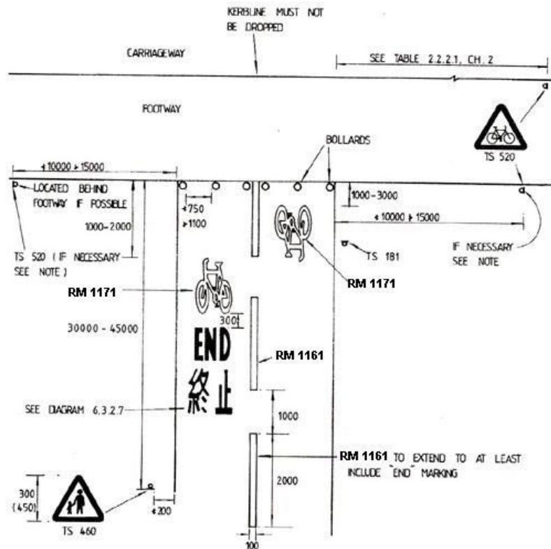
DIAGRAM 6.3.2.4 : TERMINATION OF CYCLE TRACK AT BACK OF FOOTWAY
