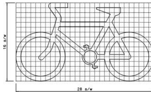
DIAGRAM 3.5.7.38 : CYCLE SYMBOL
