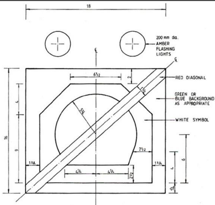
DIAGRAM 4.5.5.2 : DETAILED DIMENSIONS OF "TUNNEL CLOSED" SYMBOLIC SIGN
