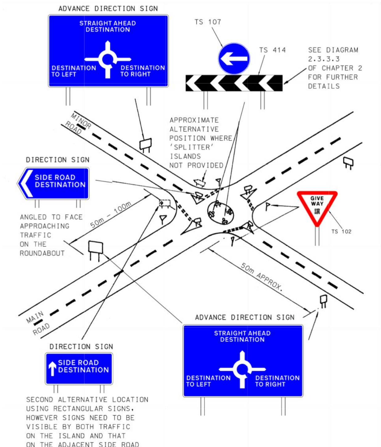
DIAGRAM 3.4.3.10 : USE OF ADVANCE DIRECTION AND DIRECTION SIGNS AT ROUNDABOUTS
