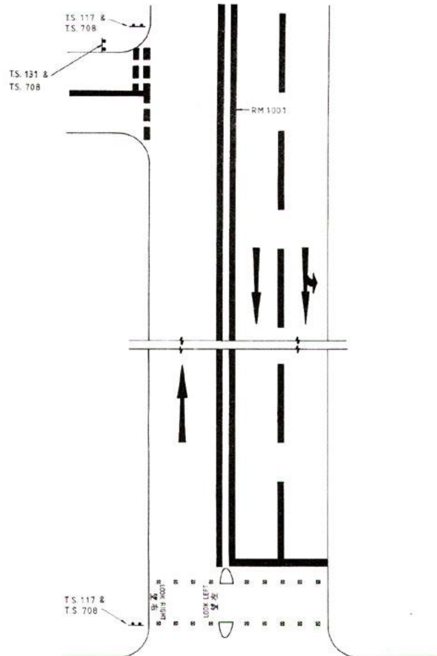
DIAGRAM 5.9.3.2 : CONTRA FLOW LANE FOR BUSES
