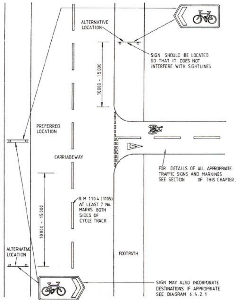
DIAGRAM 6.4.3.1 : LOCATION OF DIRECTION SIGNS NEAR START OF CYCLE TRACK
