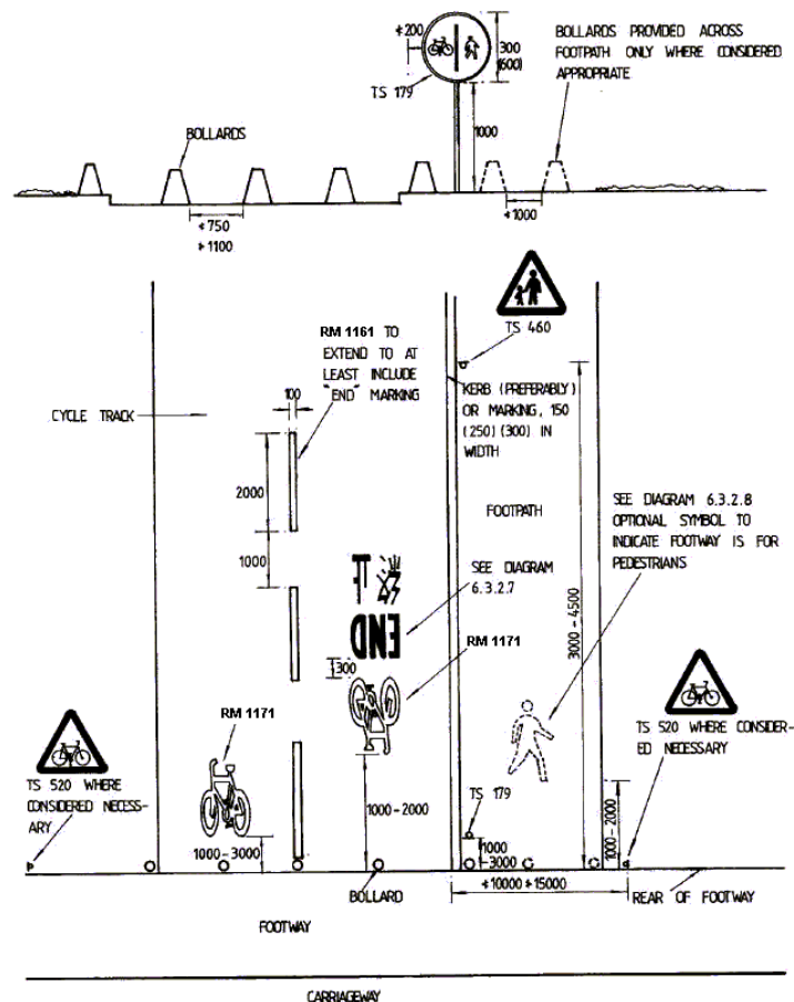
DIAGRAM 6.3.2.5 : TERMINATION / COMMENCEMENT OF CYCLE TRACK / FOOTPATH AT BACK OF FOOTWAY
