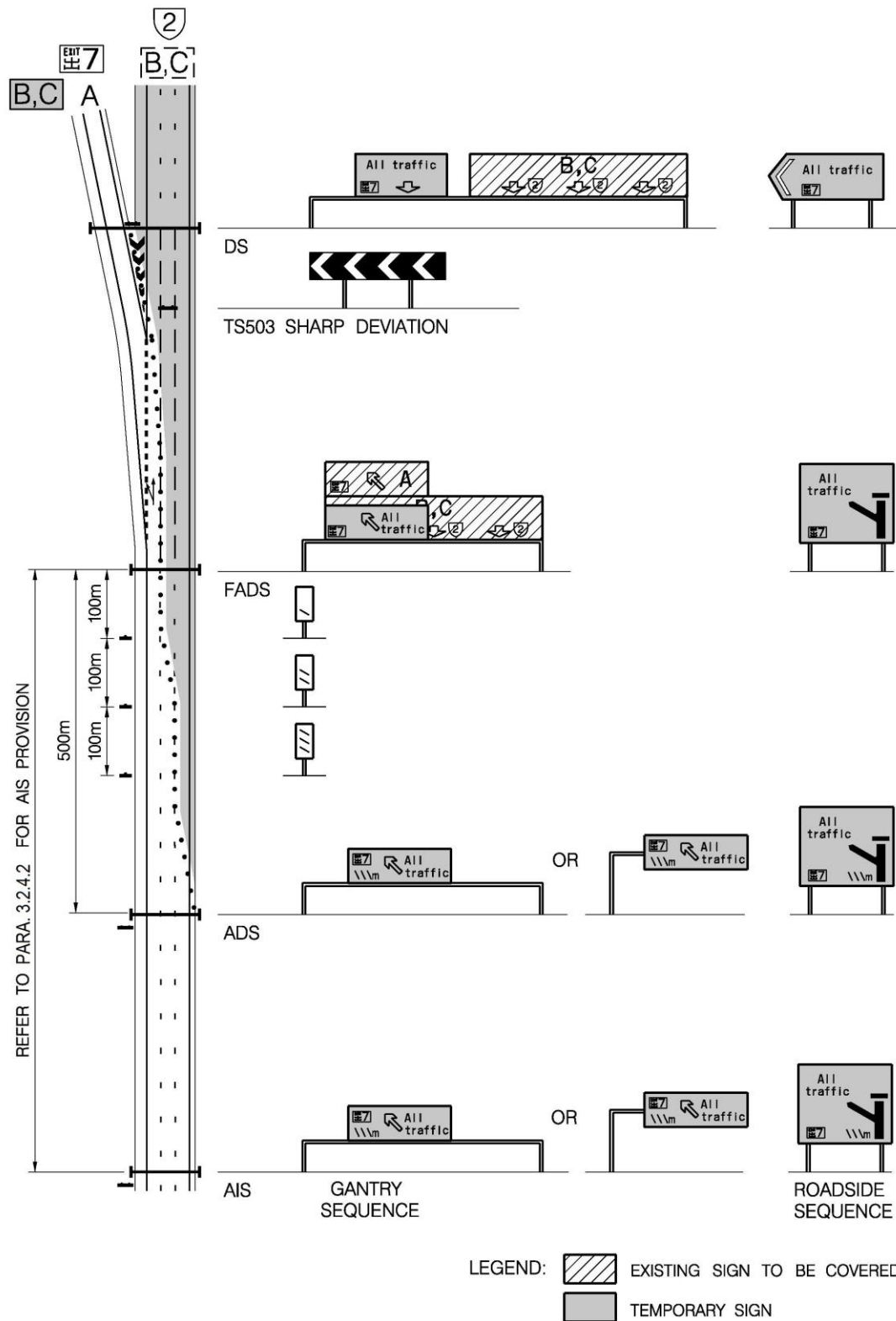
DIAGRAM 3.6.8.1 : SIGNING SCHEME FOR MAINLINE CLOSURE AT TAPER DIVERGE JUNCTION
