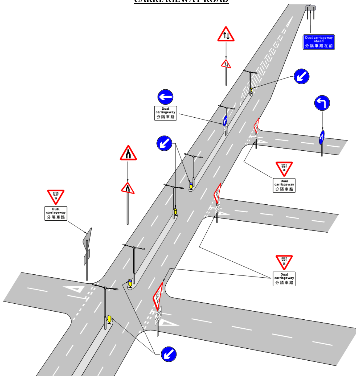
DIAGRAM 2.3.3.1 : SIGNING ARRANGEMENTS AT JUNCTIONS WITH A DUAL CARRIAGEWAY ROAD
