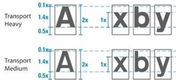
DIAGRAM 7.3.2.6 : x-HEIGHT
