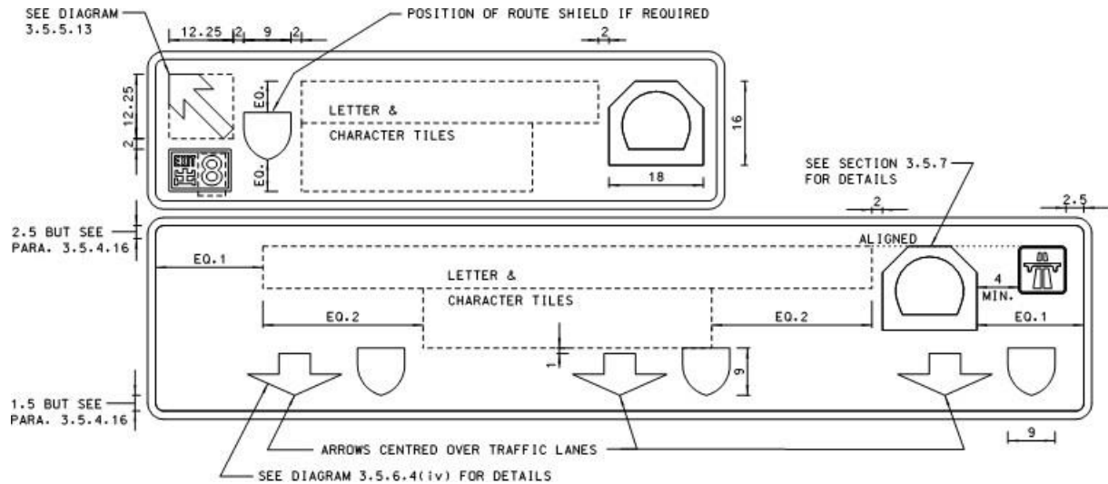
DIAGRAM 3.5.6.10 : "LANE DROP" FINAL ADVANCE DIRECTION SIGN DIMENSIONS IN STROKE WIDTHS
