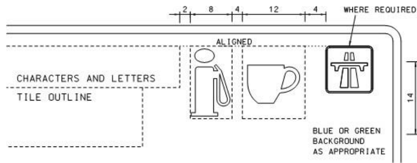
DIAGRAM 3.5.7.42 : USE OF SERVICE AREA SYMBOLS ON GANTRY SIGNS DIMENSIONS IN STROKE WIDTHS
