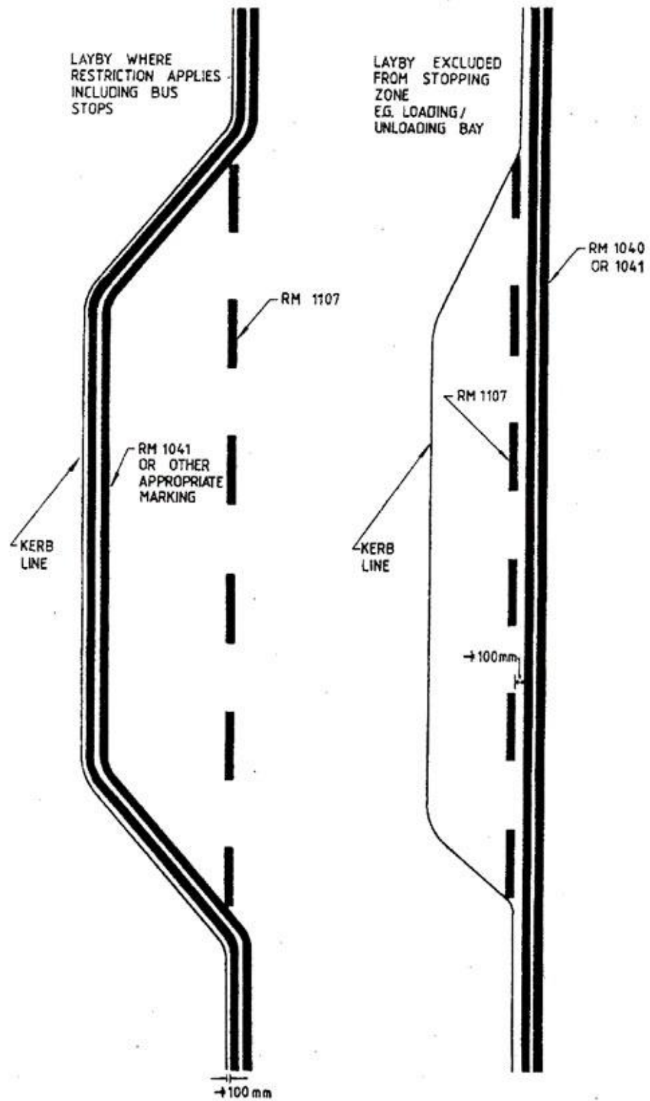
DIAGRAM 5.3.2.12 : STOPPING RESTRICTION MARKINGS AT LAYBYS
