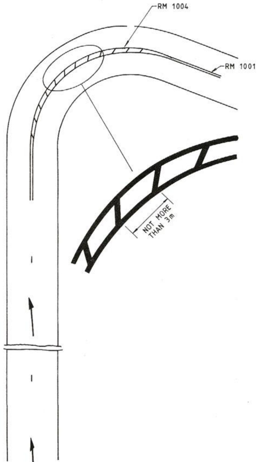
DIAGRAM 5.3.2.2 : DOUBLE LINES ON SHARP BENDS
