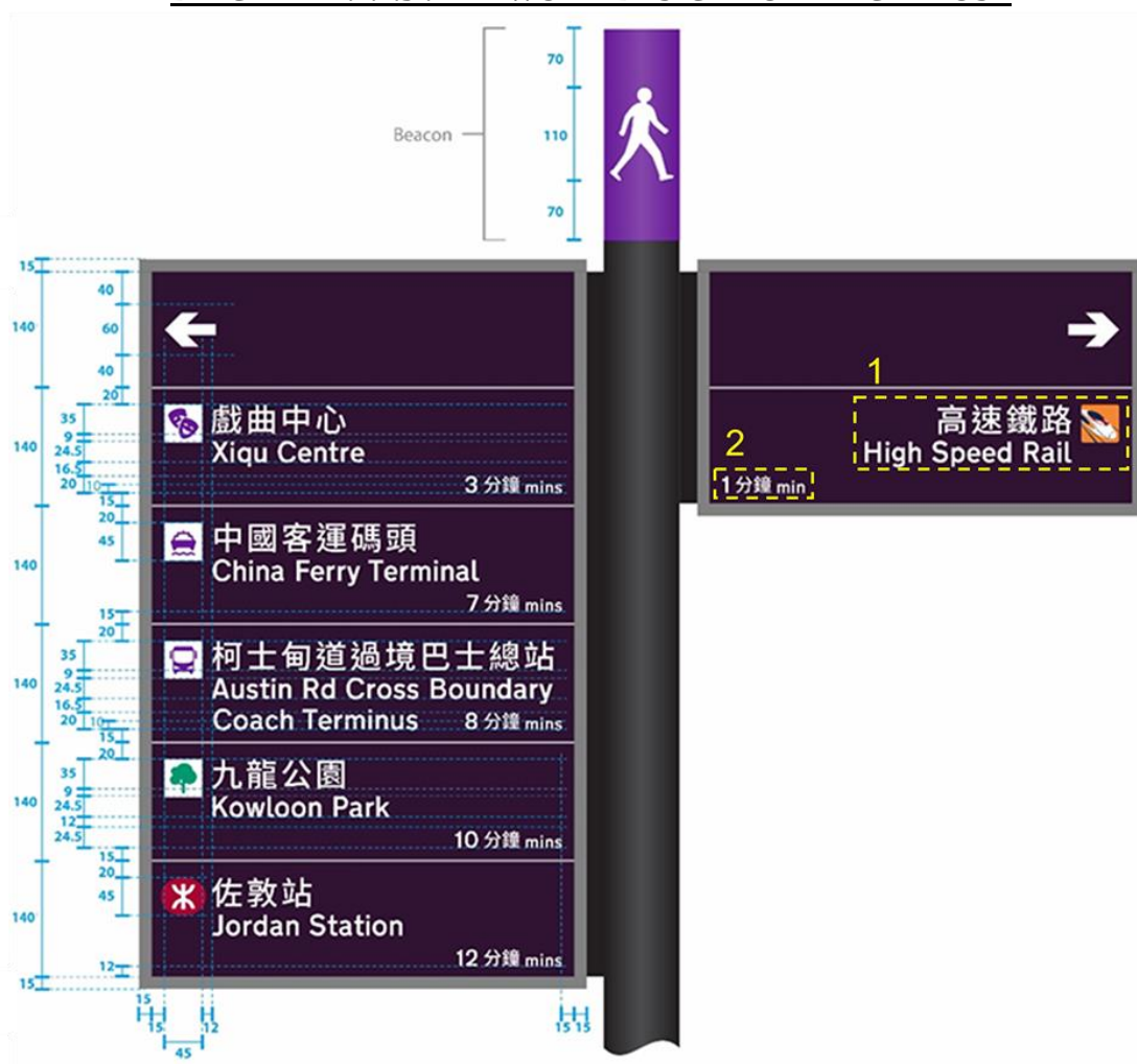
DIAGRAM 7.4.2.3 : ARTWORK DESIGN FOR FINGERPOST
