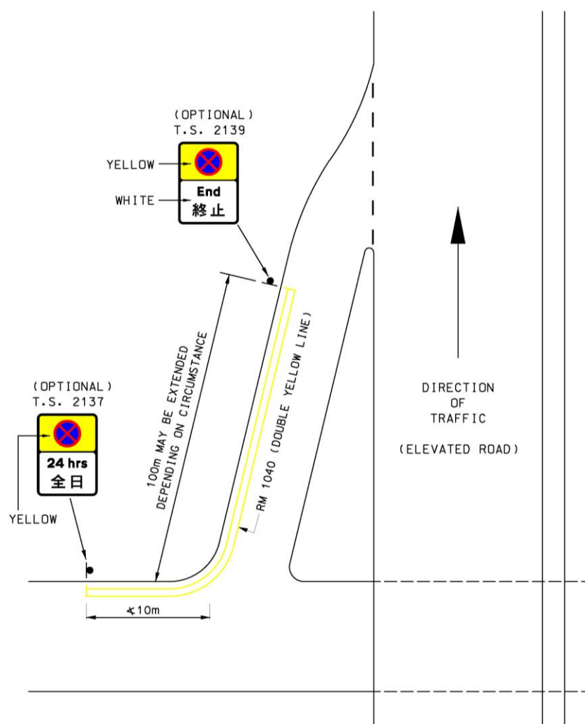
DIAGRAM 2.3.2.6 : SIGNING AND MARKING OF NO STOPPING RESTRICTIONS ON SLIP ROADS
