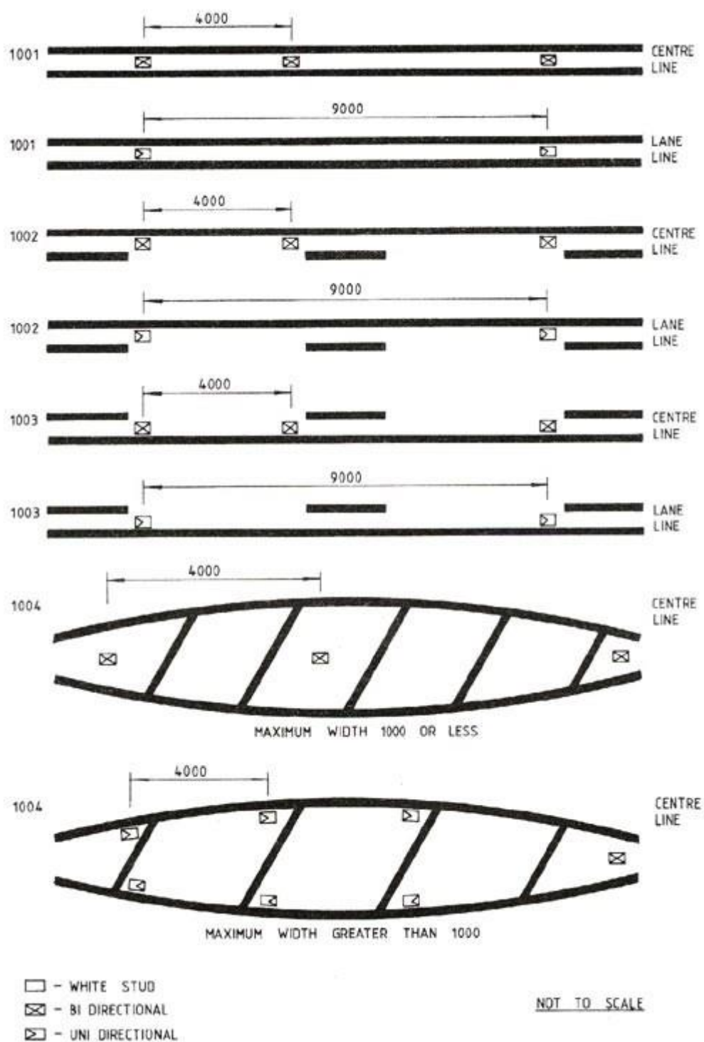
DIAGRAM 5.5.3.1 : STUDS FOR DOUBLE WHITE LINES - SINGLE CARRIAGEWAY ROAD
