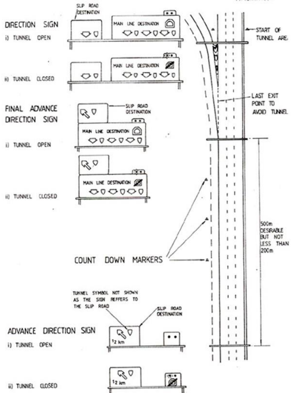
DIAGRAM 4.5.5.10 : USE OF "TUNNEL CLOSED" SIGN ON GANTRIES
