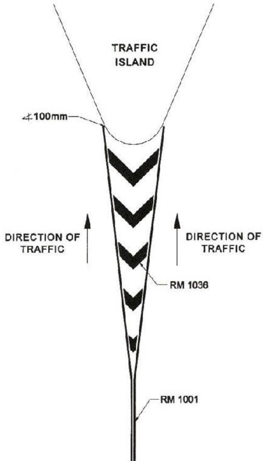
DIAGRAM 5.3.2.8 : DOUBLE LINES AT TRAFFIC ISLAND ON ONE WAY CARRIAGEWAY
