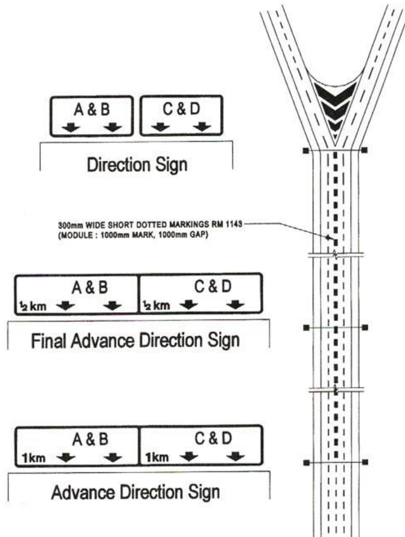
DIAGRAM 5.4.2.4(B) : 300mm WIDE SHORT DOTTED MARKINGS ON EXPRESSWAY TO DELINEATE LANE DROP
