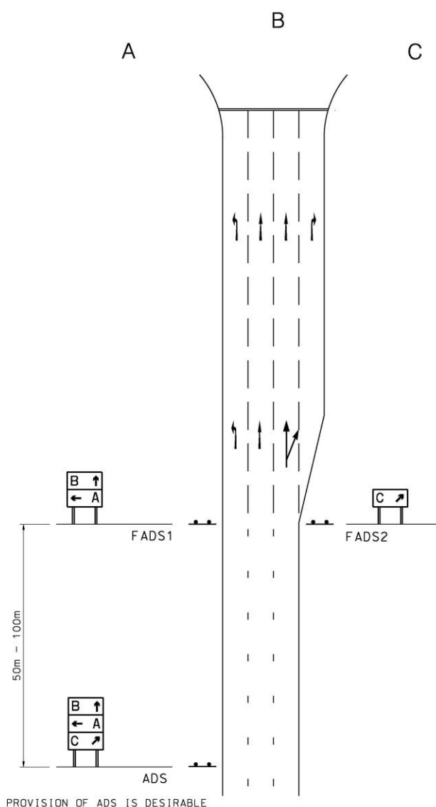
DIAGRAM 3.4.3.8 : SPLIT DIRECTION SIGNS AT SIGNAL CONTROLLED INTERSECTIONS
