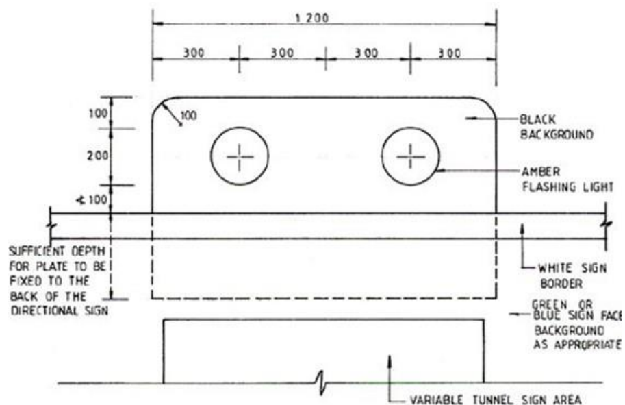
DIAGRAM 4.5.5.3 : LOCATION AND DETAILS OF AMBER FLASHING LIGHTS ON GANTRY SIGNS AND ON CERTAIN ROAD SIDE SIGNS
