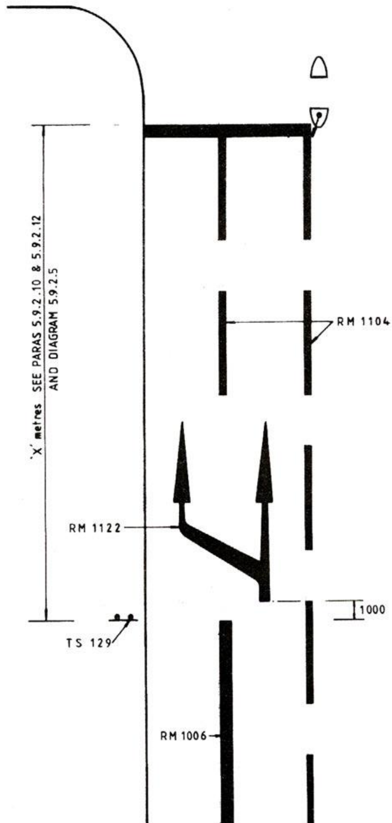
DIAGRAM 5.9.2.4 : END OF BUS LANE MARKINGS
