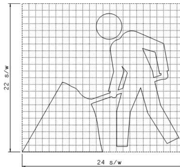
DIAGRAM 3.5.7.33: ROAD WORKS AHEAD SYMBOL FOR DIRECTION SIGNS DIMENSIONS IN STROKE WIDTHS
