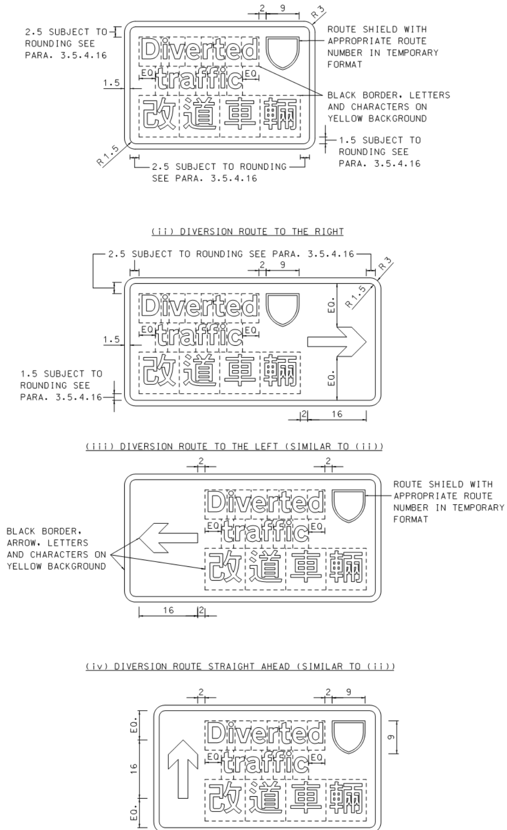
DIAGRAM 3.6.8.7 : ROADSIDE "DIVERSION" SIGNS WITH ROUTE SHIELD DIMENSIONS IN STROKE WIDTHS
