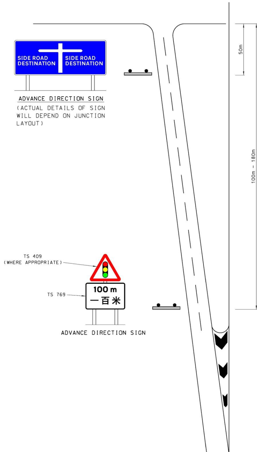
DIAGRAM 3.4.2.24: SLIP ROAD DIRECTIONAL SIGNING PRIORITY / TRAFFIC SIGNAL JUNCTION
