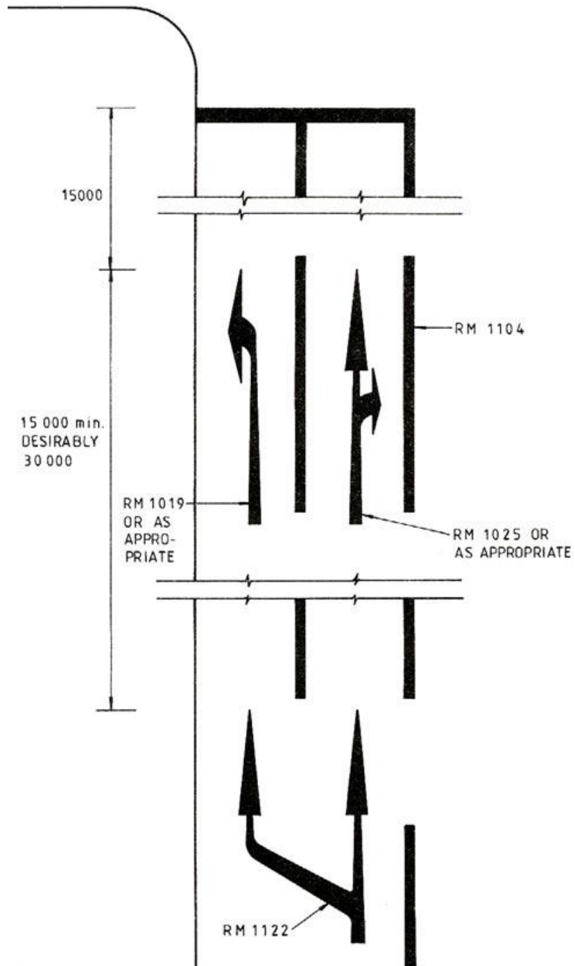
DIAGRAM 5.9.2.5 : MINIMUM SETBACK OF BUS LANE IN RESPECT OF NECESSARY DIRECTION ARROW MARKINGS
