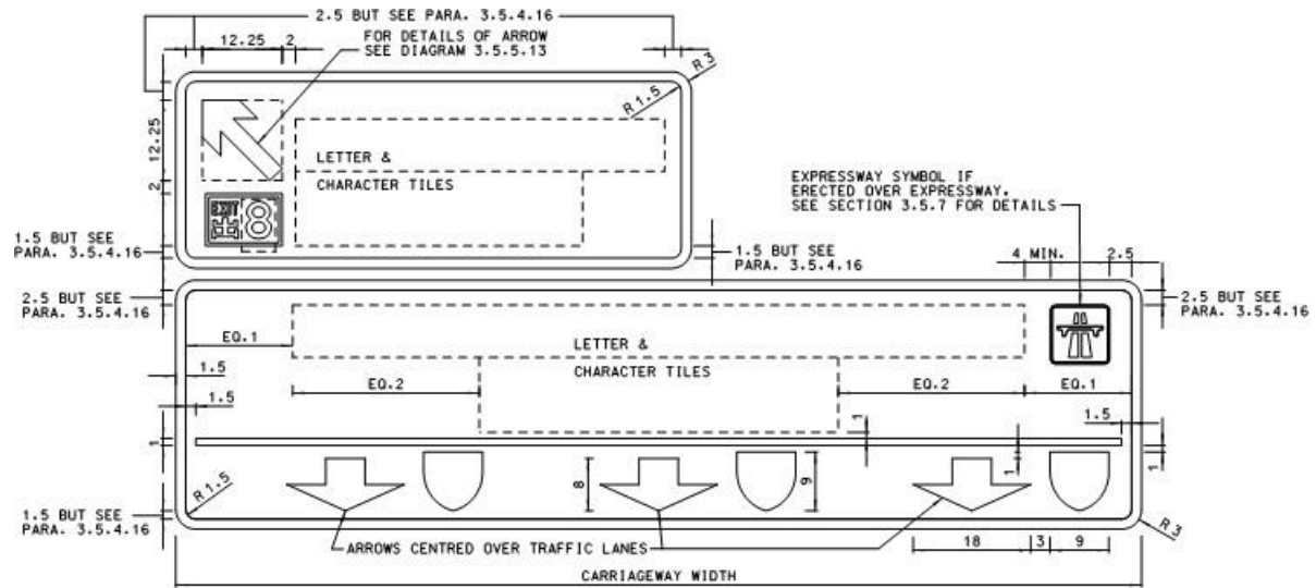
DIAGRAM 3.5.6.7 : FINAL ADVANCE DIRECTION SIGN DESIGN DETAILS DIMENSIONS IN STROKE WIDTHS
