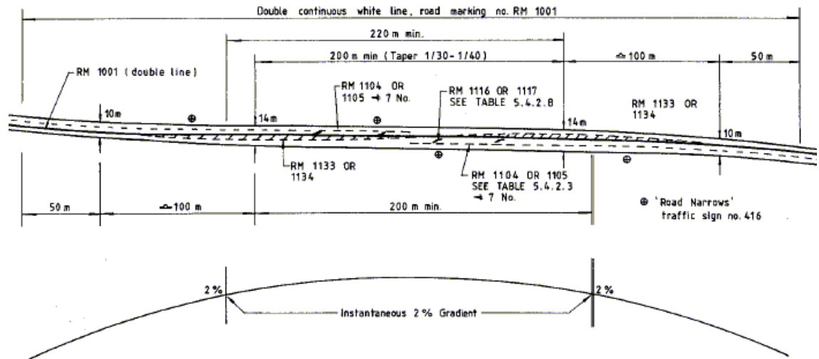
DIAGRAM 5.3.2.5 : MARKINGS FOR CREST CURVE BETWEEN CLIMBING LANES ( SEE ALSO SECTION 3.3.8 CHAPTER 3 VOLUME 2 )
