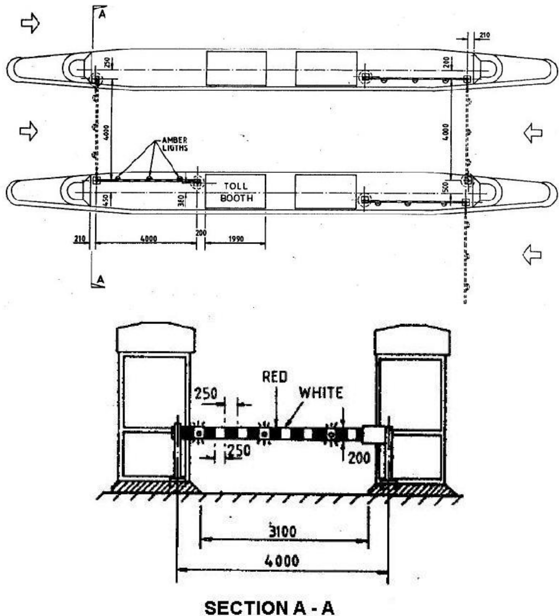
DIAGRAM 4.6.1.4 : BARRIERS AT TOLL BOOTHS
