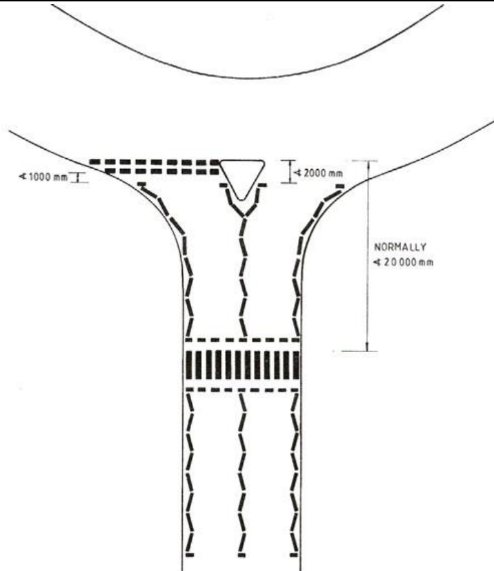
DIAGRAM 5.7.2.5 : ZEBRA CROSSING NEAR ROUNDABOUT
