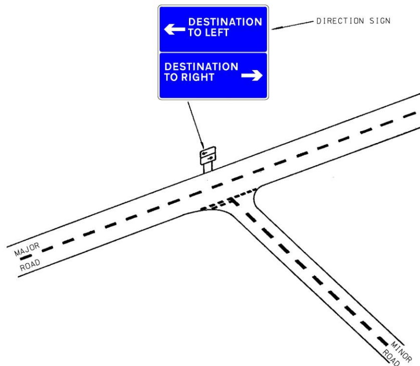
DIAGRAM 3.4.3.16 : DIRECTION SIGN FOR MINOR ROAD ONLY
