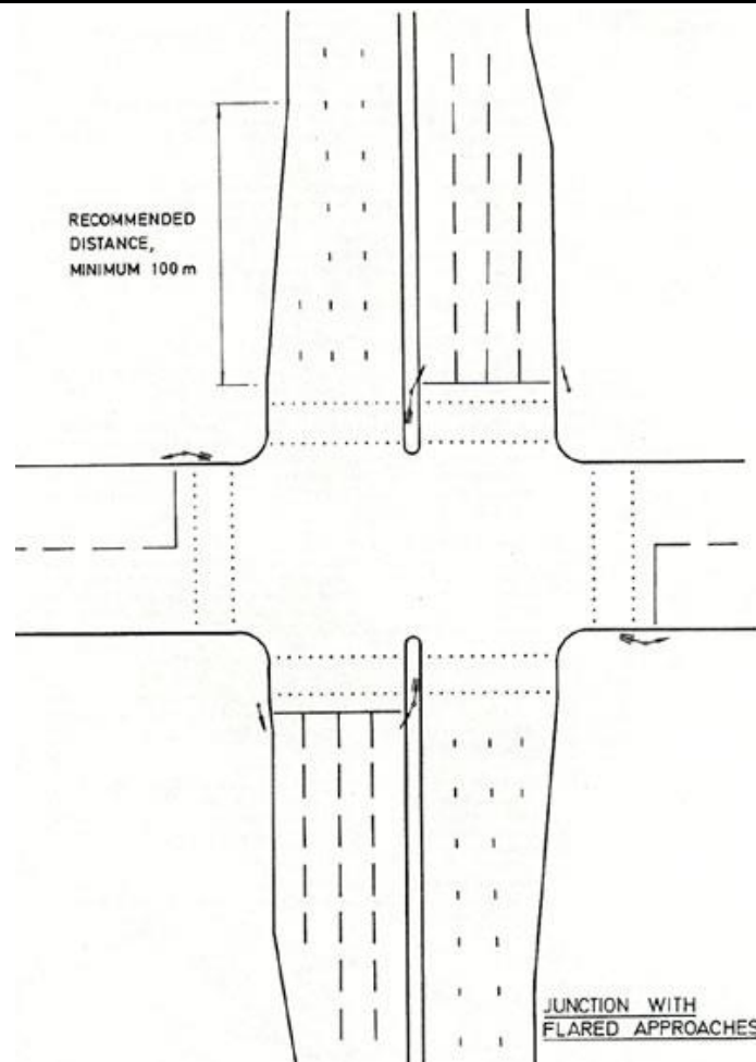
DIAGRAM 2.2.3.5 : JUNCTION WITH FLARED APPROACHES
