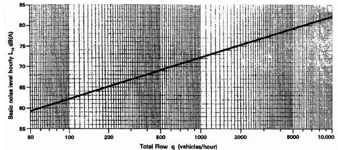
DIAGRAM 7.4.2.2 : PREDICTION OF BASIC NOISE LEVEL HOURLY L10 IN TERMS OF TOTAL HOURLY FLOW q ( V=75 km/h, p=0 , G=0 )
