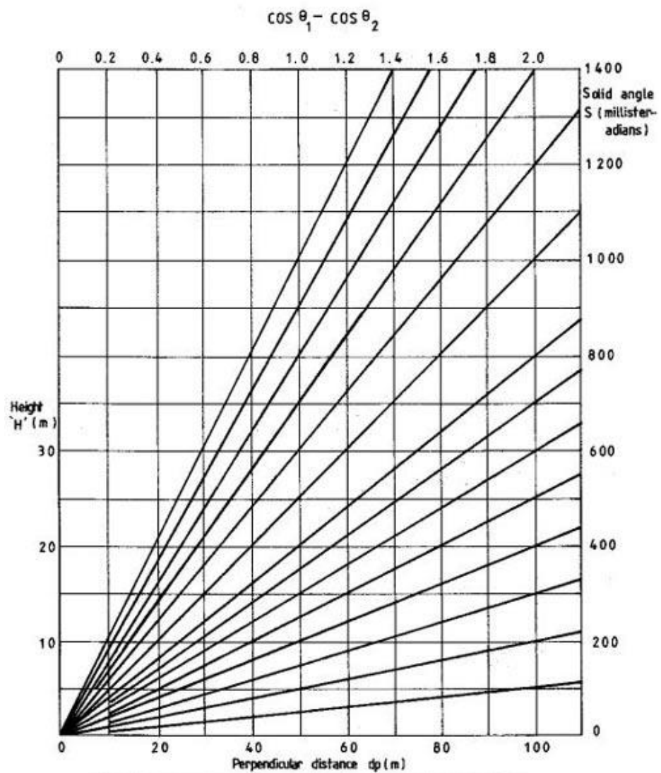
USE OF SOLID ANGLE PREDICTION CHART
