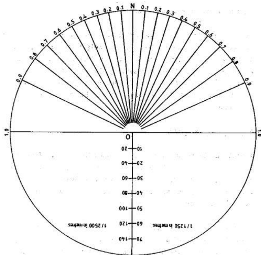
DIAGRAM 7.5.2.2 : SIMPLIFIED SOLID ANGLE PROTRACTOR
