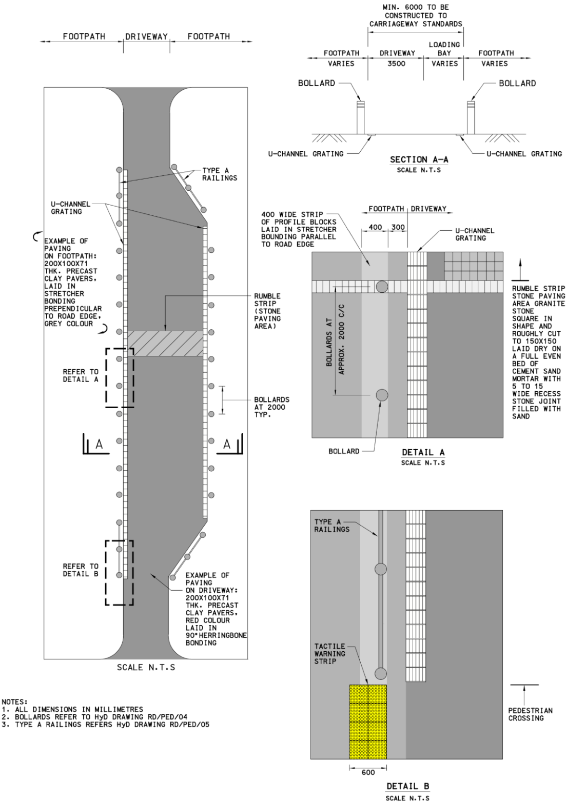
DIAGRAM 10.5.3.2: EXAMPLE OF SHARED SURFACE STREET
