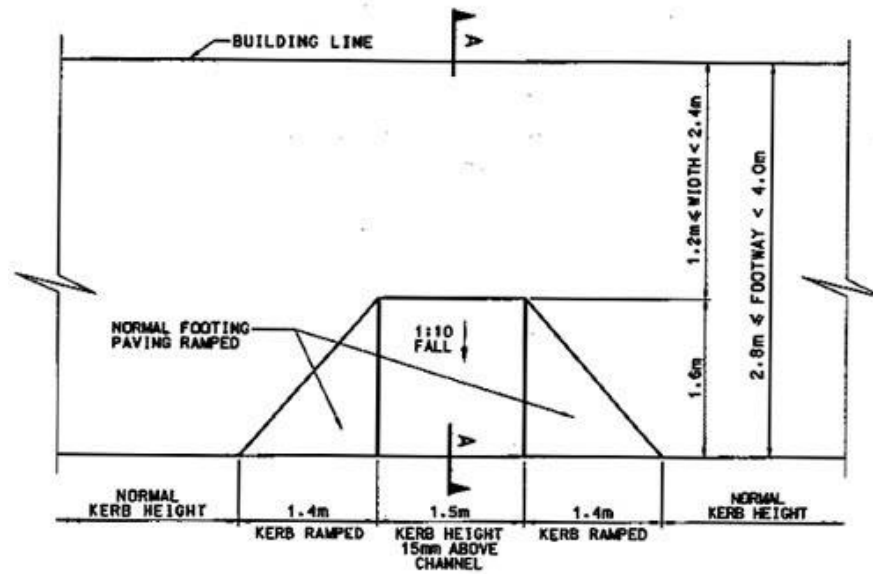
DIAGRAM 8.8.2.2 : TAXI STAND WITH ACCESS RAMP FOR PEOPLE WITH DISABILITIES ( 2.8\text{m} \leq \text{FOOTWAY} < 4.0\text{m} )
