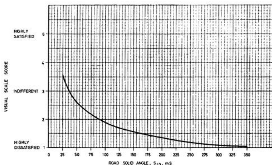
DIAGRAM 7.5.3.1 : VISUAL JUDGEMENTS VERSUS ROAD SOLID ANGLE
