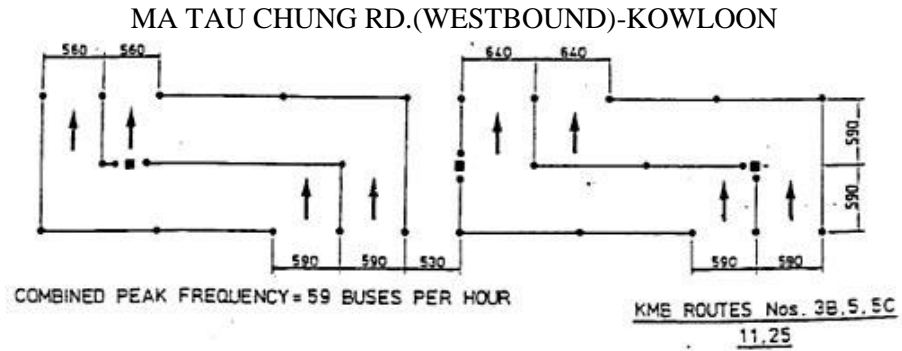
DIAGRAM 2.6.3.4: PREVIOUS BUS QUEUE RAILING ARRANGEMENTS FOR TYPE 'A' BUS SHELTERS FOR ADJACENT STOPS (NOT RECOMMENDED) SCALE 1:100 ALL DIMENSIONS IN MILLIMETERS
