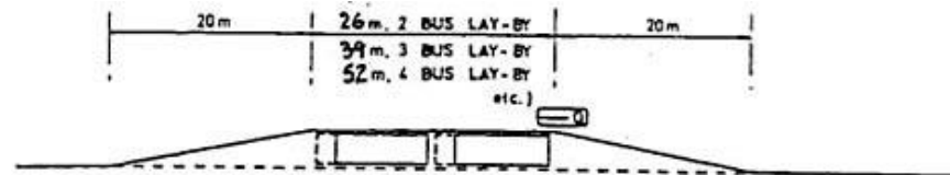
DIAGRAM 2.5.4.2: STANDARD MULTI-BUS LAY-BY
