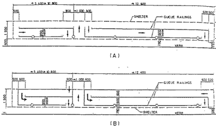
DIAGRAM 2.6.3.4: PREVIOUS BUS QUEUE RAILING ARRANGEMENTS FOR TYPE 'A' BUS SHELTERS FOR ADJACENT STOPS (NOT RECOMMENDED) SCALE 1:100 ALL DIMENSIONS IN MILLIMETERS
