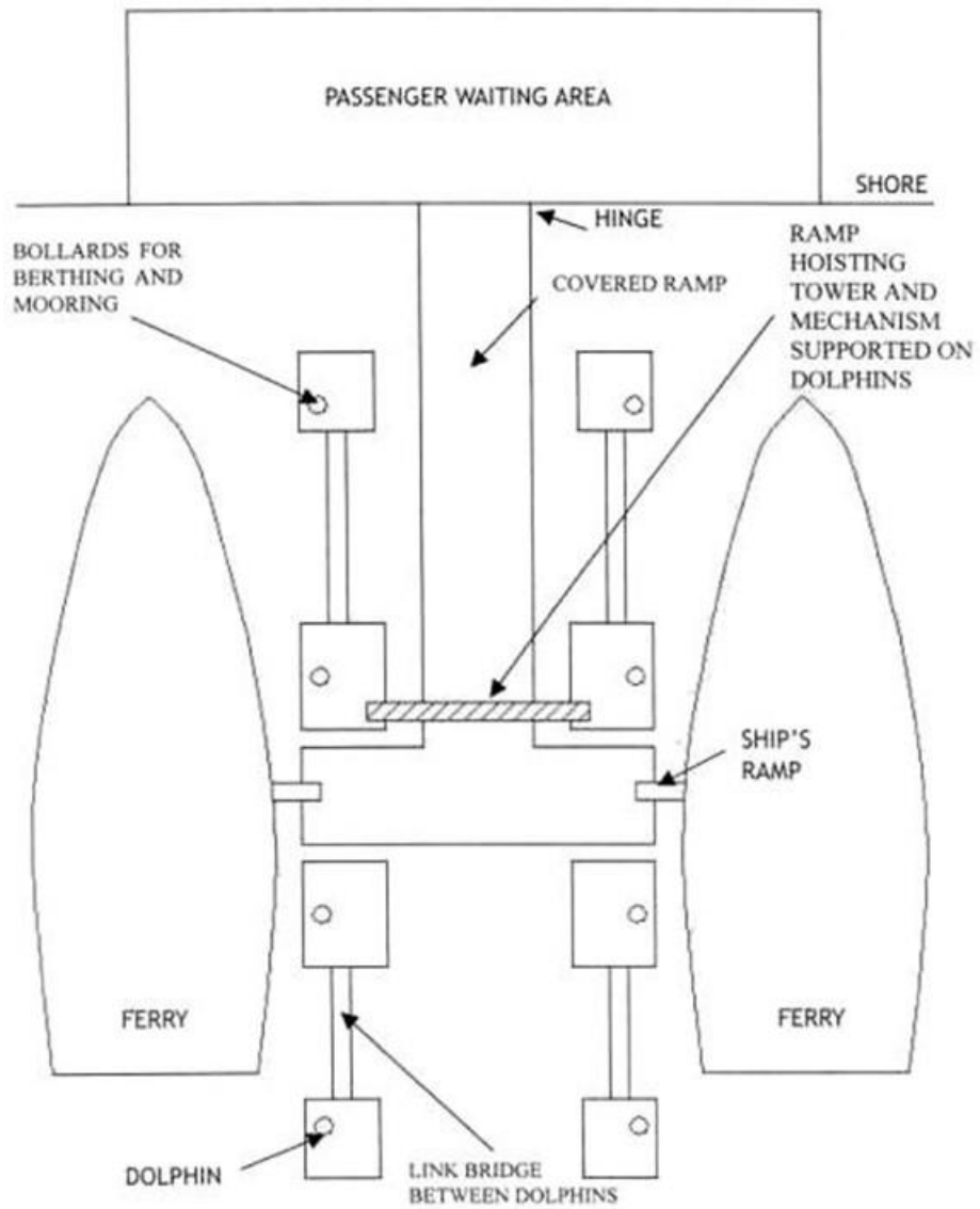
Typical Linkspan Arrangement (Two Berths)
