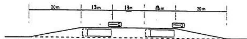
DIAGRAM 2.5.4.3: STANDARD SINGLE-BUS/MULTI-STOP LAY -BY
