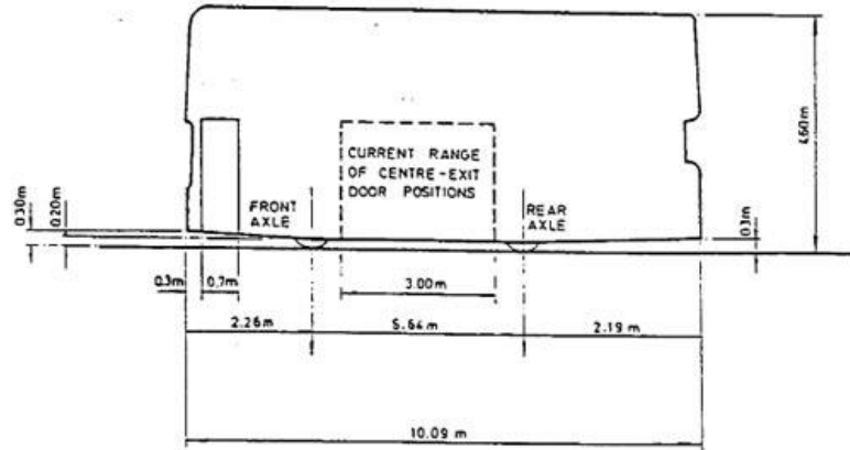
DIAGRAM 2.3.5.1: BODY PROFILE FOR THE DESIGN 2 AXLE BUS SCALE:1:100
