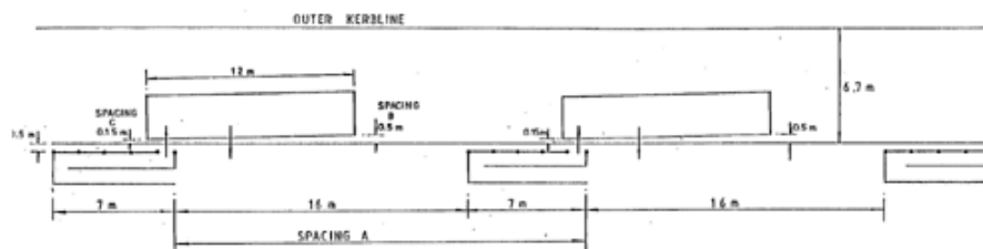
DIAGRAM 2.6.3.5: SETTING OUT DETAILS FOR STANDARD QUEUE RAILING AT ADJACENT STOPS SCALE 1:200
