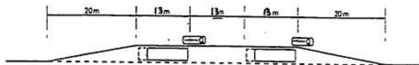
DIAGRAM 2.5.4.4: OPEN-ENDED LAY-BY
