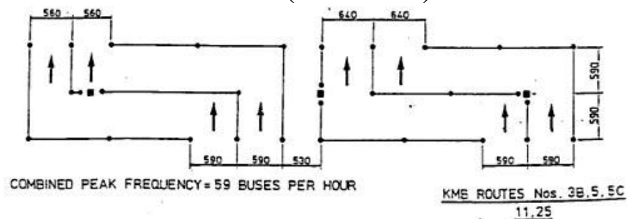
DIAGRAM 2.6.3.4: PREVIOUS BUS QUEUE RAILING ARRANGEMENTS FOR TYPE 'A'
