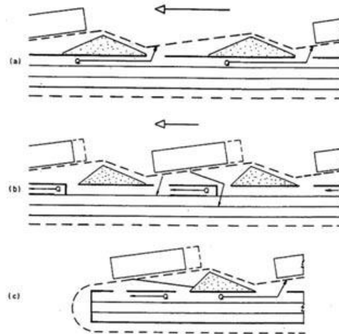
DIAGRAM 2.7.14.8: ALTERNATIVE PASSENGER QUEUING ARRANGEMENTS
