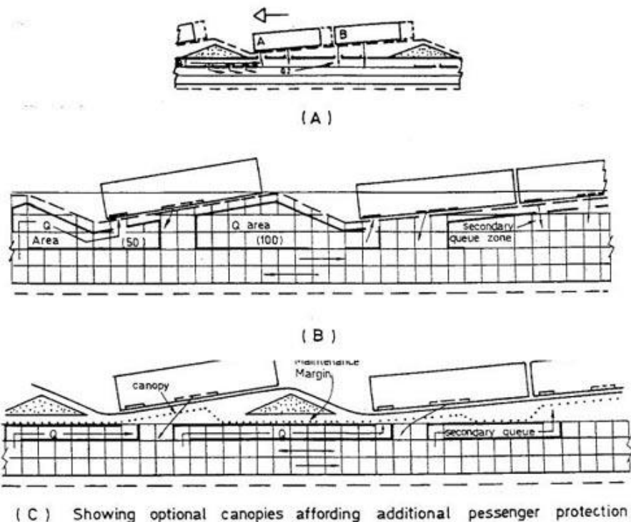
DIAGRAM 2.7.14.13: ALTERNATIVE PASSENGER QUEUING ARRANGEMENTS
