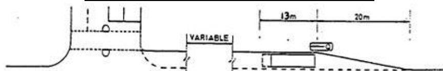
DIAGRAM 2.5.4.4: OPEN-ENDED LAY-BY
