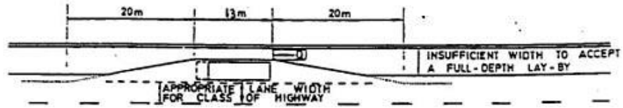
DIAGRAM 2.5.4.6: LAY-BY WITH SUB-STANDARD DEPTH
