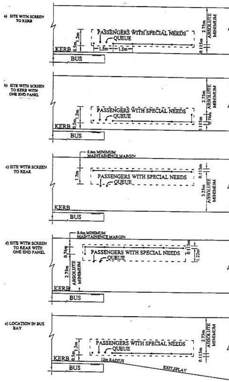
DIAGRAM 2.6.3.1: SITING ARRANGEMENTS FOR CANTILEVER SHELTERS WITHOUT QUEUE RAILINGS
