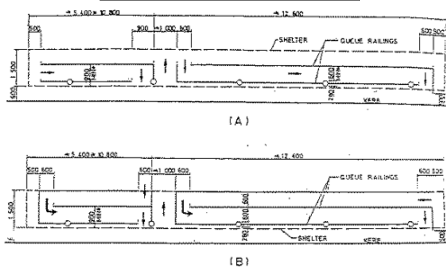
DIAGRAM 2.6.3.5: SETTING OUT DETAILS FOR STANDARD QUEUE RAILING AT
