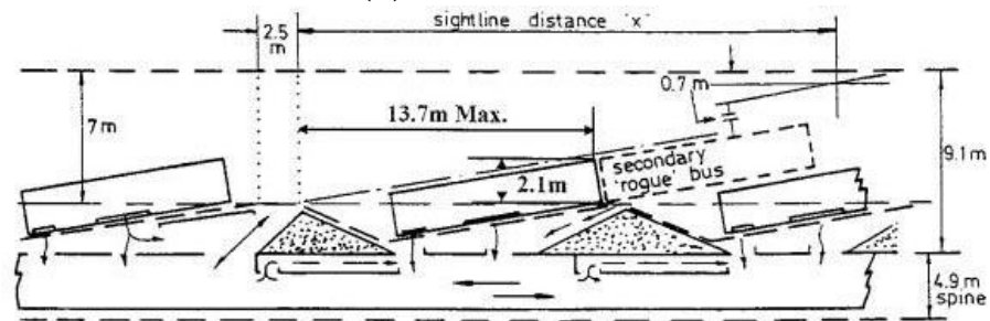
(B) Shallow Sawtooth
