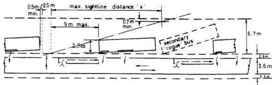
(A) Linear Stands
