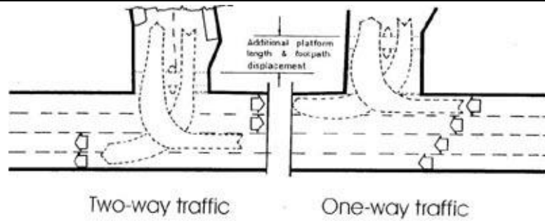
DIAGRAM 2.7.14.6: ENTRANCE/EXIT PATHS FROM TWO-WAY BUS STATION LANES
