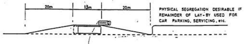
DIAGRAM 2.5.4.5: STANDARD COMBINED LAY-BY
