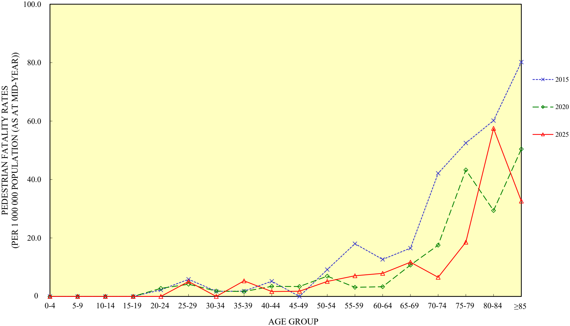
FIGURE B4 - PEDESTRIAN FATALITY RATES BY AGE GROUP IN 2015, 2020 AND 2025
