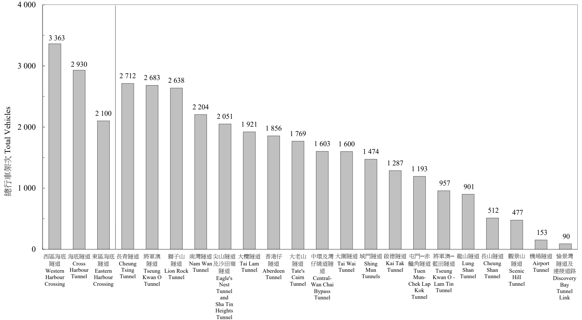
Chart 3.1 - Vehicular Flow Through Tunnels (January 2026)
