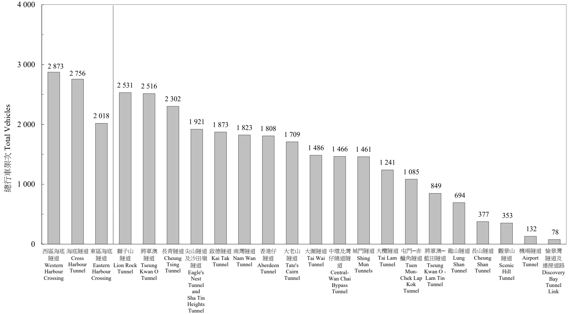
Chart 3.1 - Vehicular Flow Through Tunnels (September 2024)
